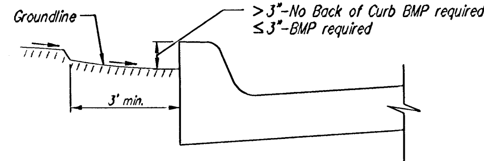
CURB BACKFILL DETAIL
