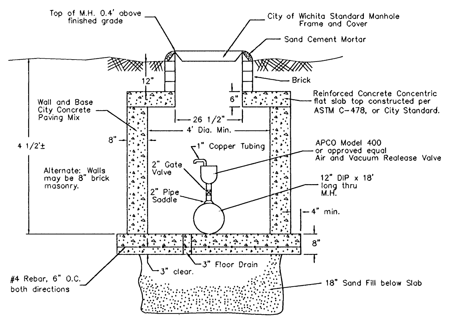
Air & Vacuum Release Detail
