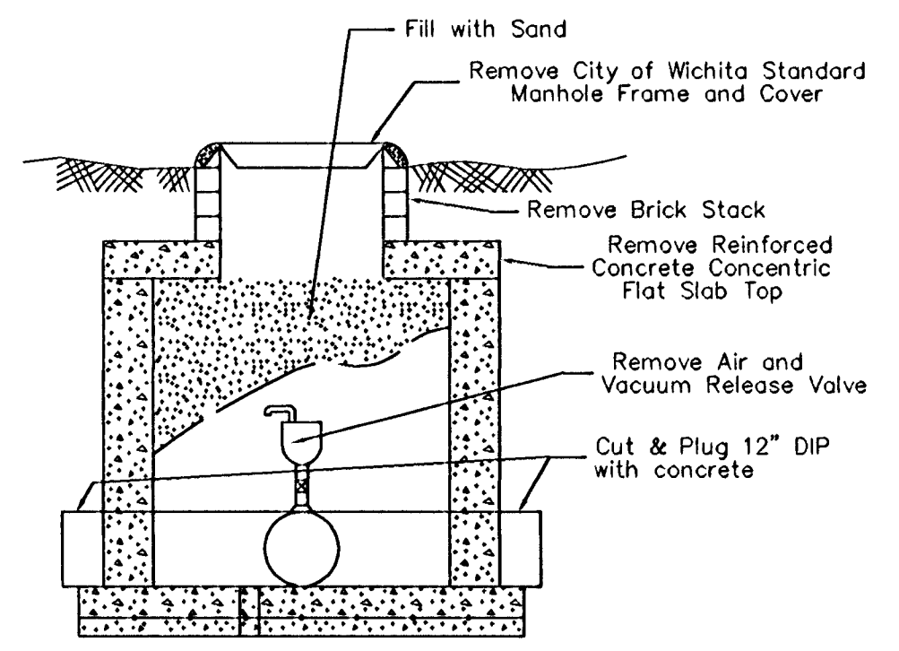
Abandon Manhole Detail
