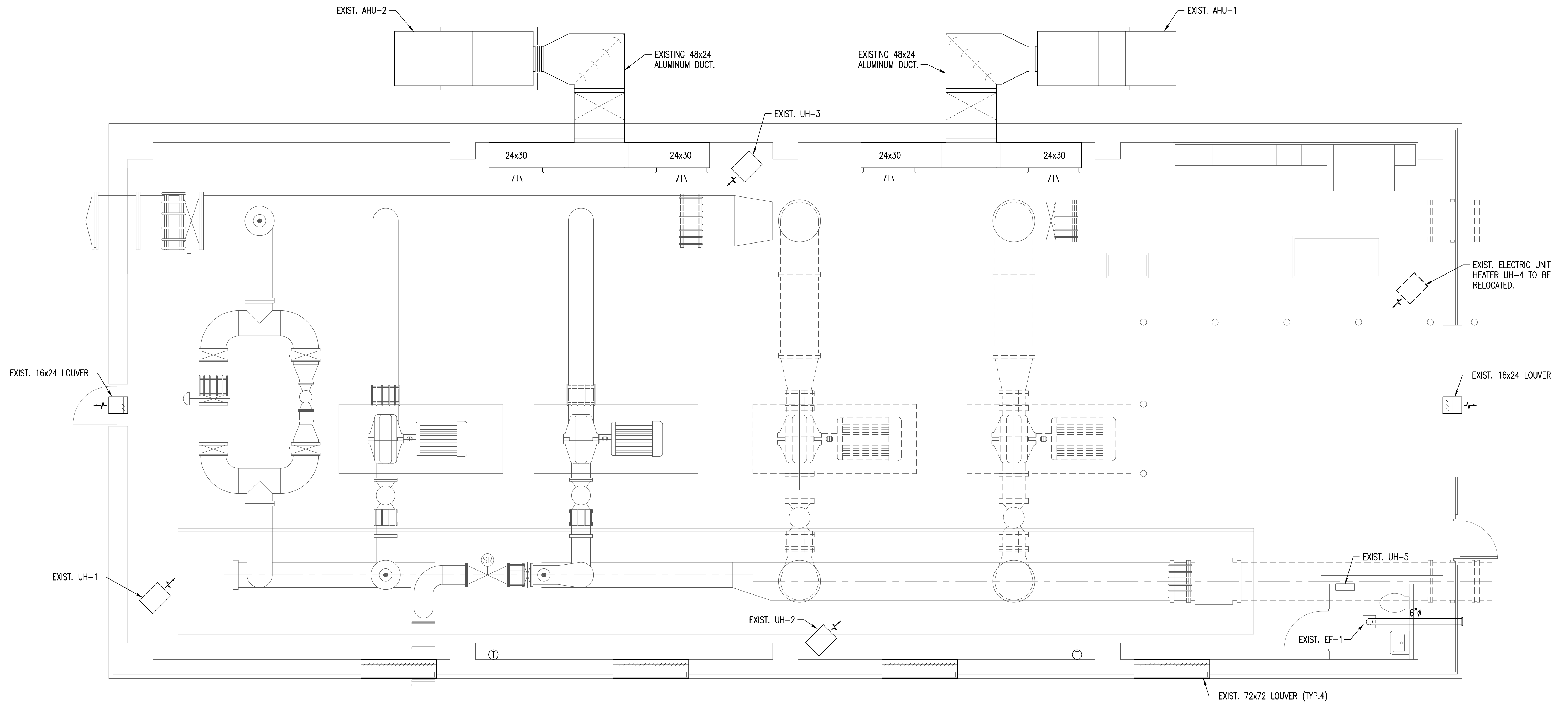
A MECHANICAL DEMOLITION FLOOR PLAN 0' 2' 4' 6' 10' SCALE: 1/4" = 1'-0"
