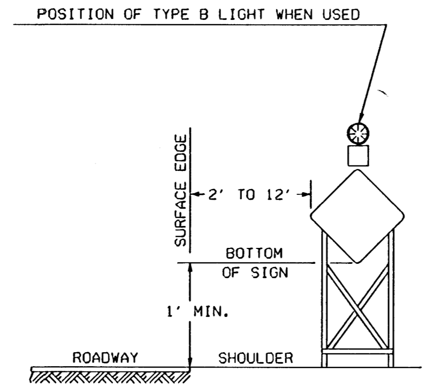
HEIGHT AND LATERAL DIMENSIONS FOR SIGNS MOUNTED ON SKIDS OR OTHER MOVABLE MOUNTS
