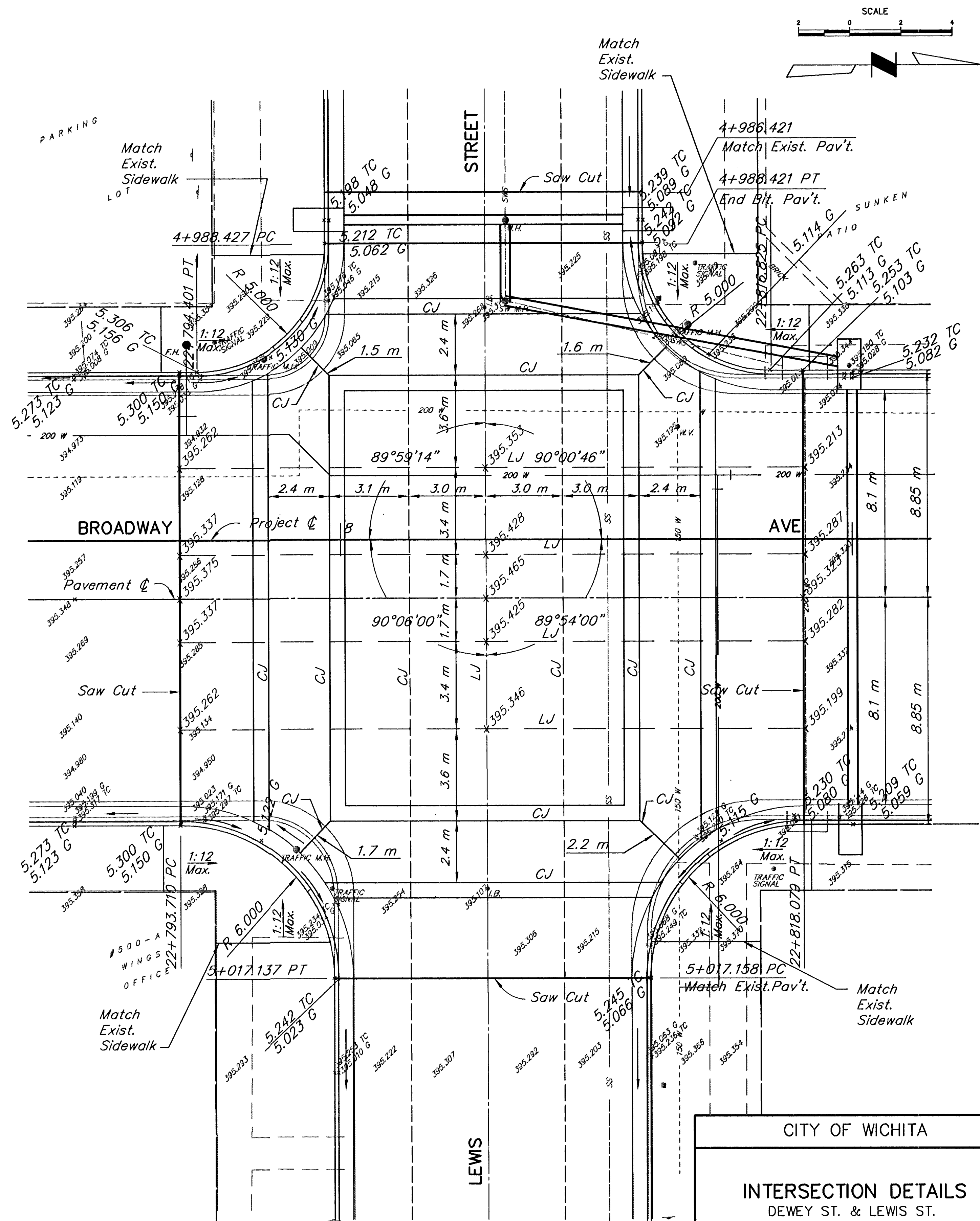
PLAN AT LEWIS STREET
