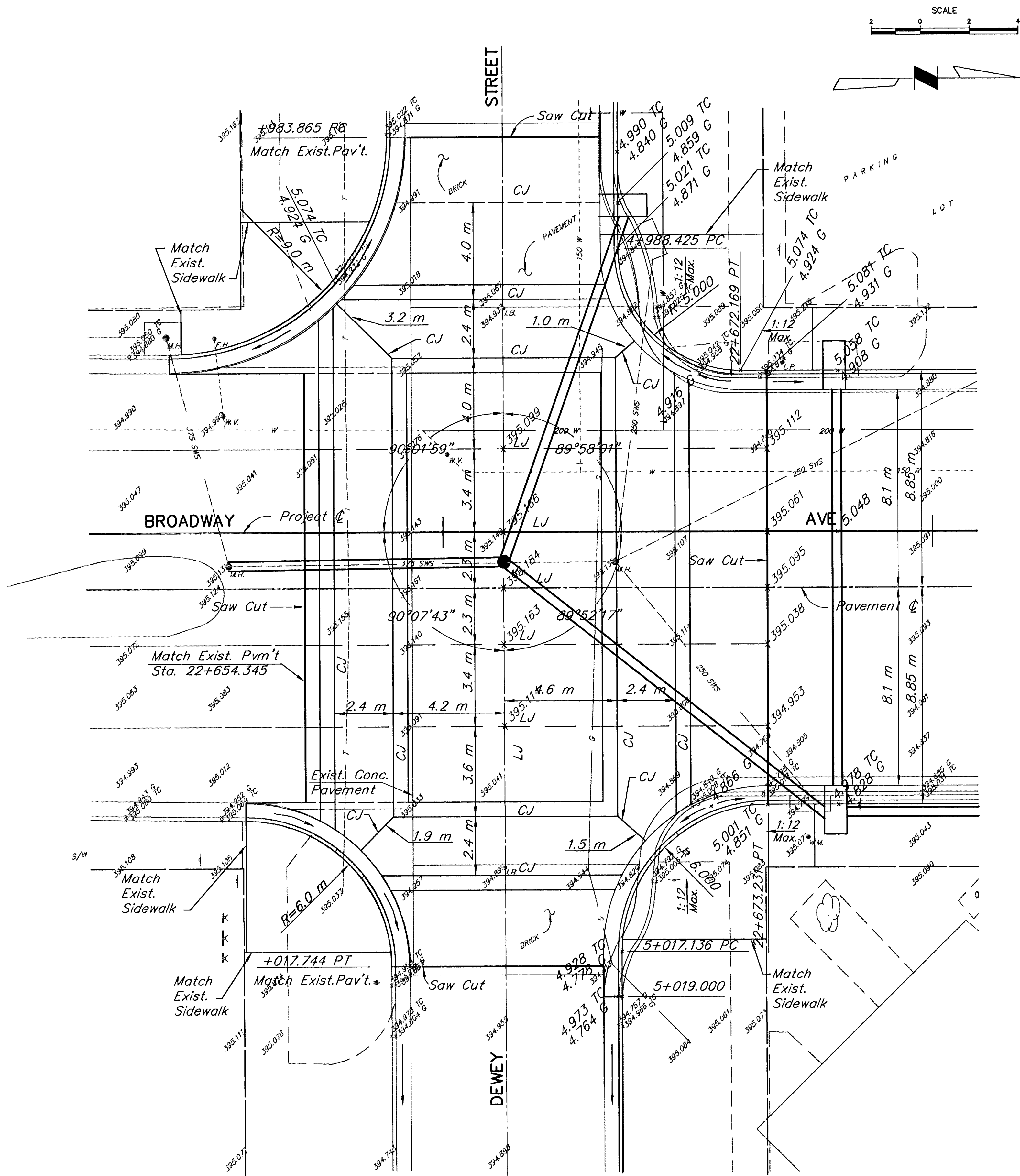
PLAN AT DEWEY STREET
