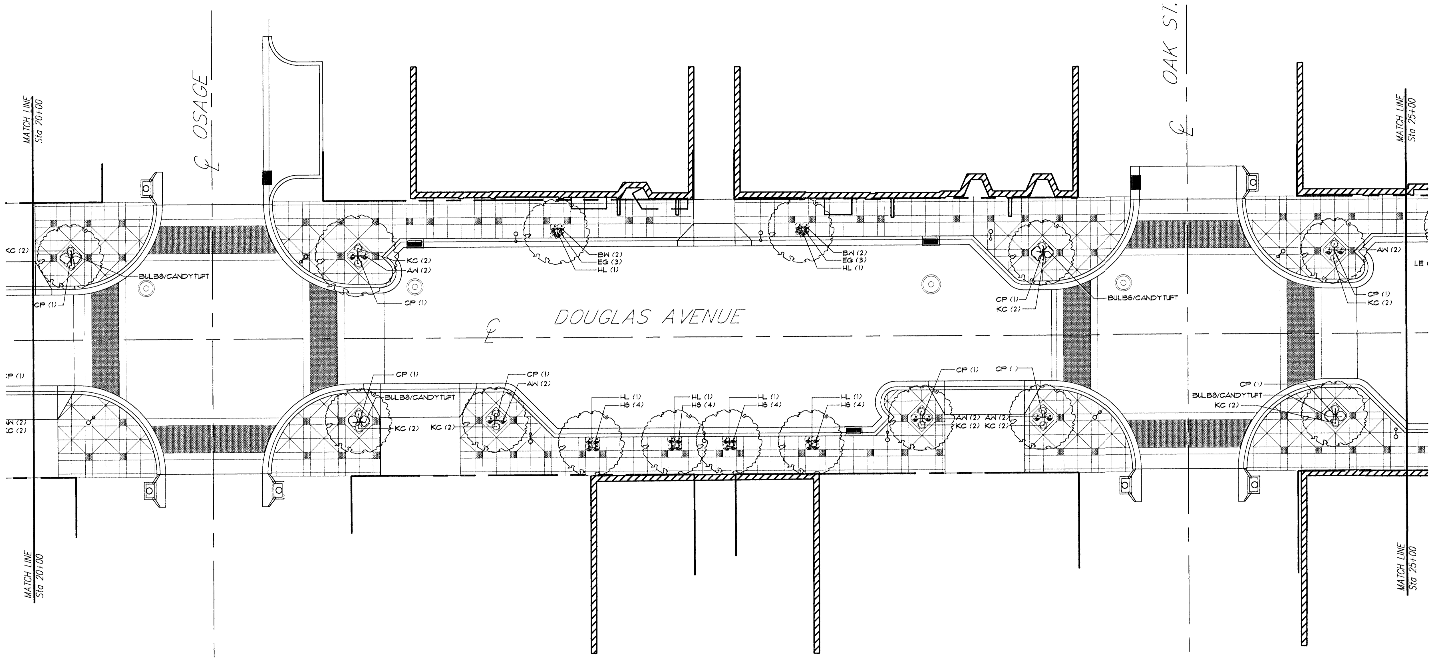
A LANDSCAPE PLAN 3 0 10' 20' 30' 50' SCALE: 1" = 20'-0" NORTH
