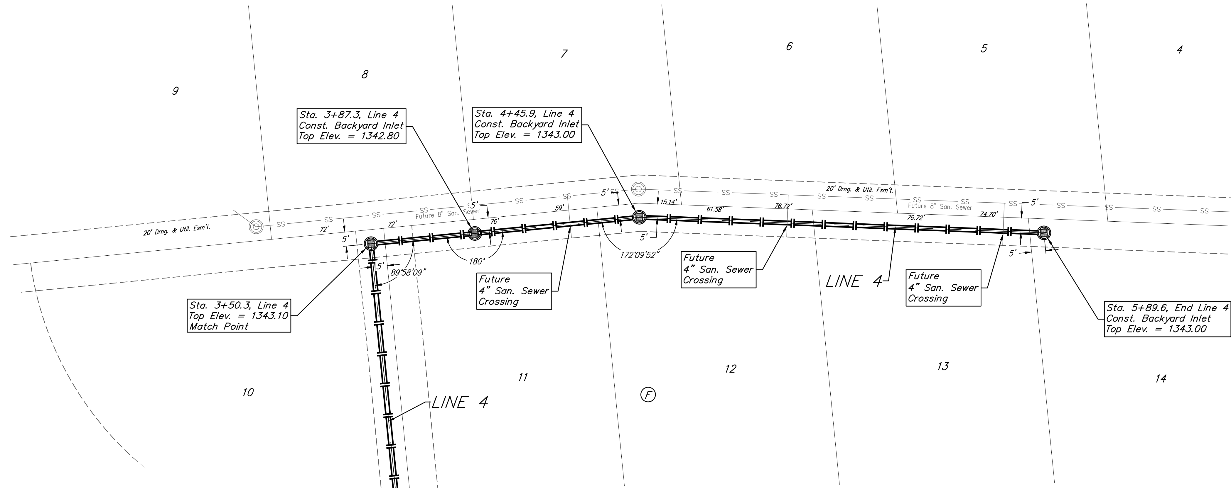
WILLOW CREEK EAST 3RD ADDITION
