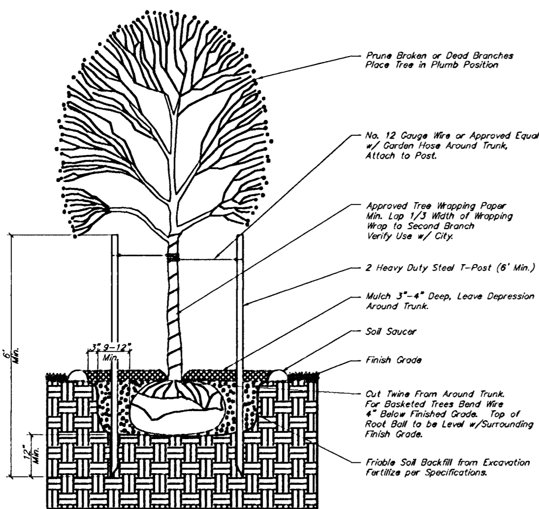
TREE PLANTING & STAKING DETAIL Deciduous Trees Larger than 2 1/2" Cal. and Smaller Evergreen Trees Larger than 6' Height No Scale
