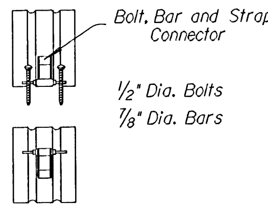
ALTERNATE CONNECTION DETAIL
