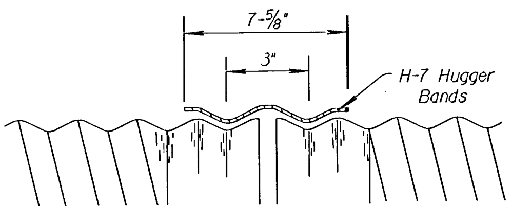
UNIVERSAL REFORMED END with H-7 HUGGER BAND DETAILS FOR H-7 HUGGER BANDS (16 ga.)
