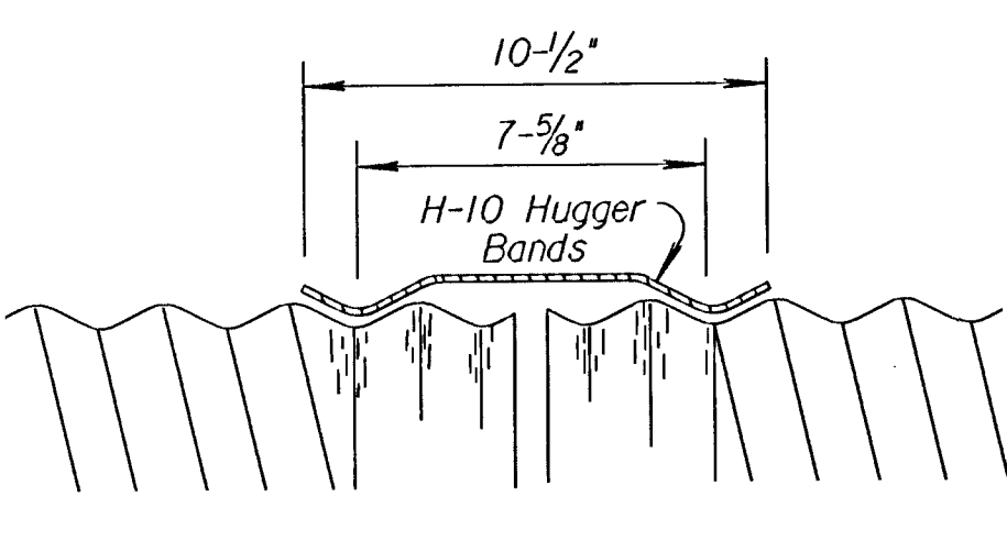
UNIVERSAL REFORMED END with H-10 HUGGER BAND DETAILS FOR H-10 HUGGER BANDS (16 ga.)
