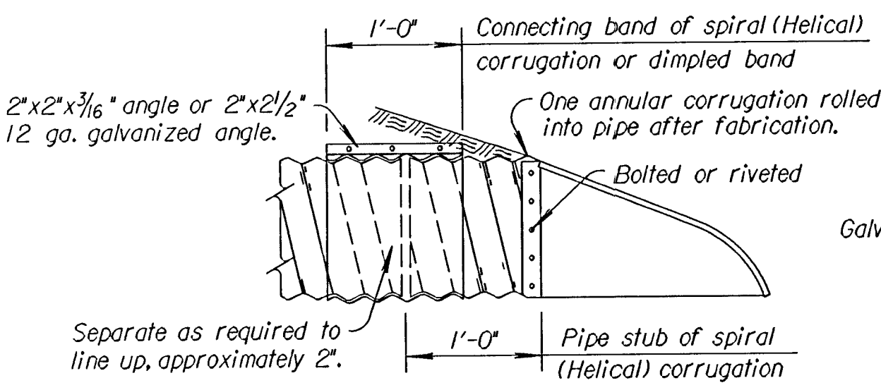
SPIRAL (HELICAL) CORRUGATION
