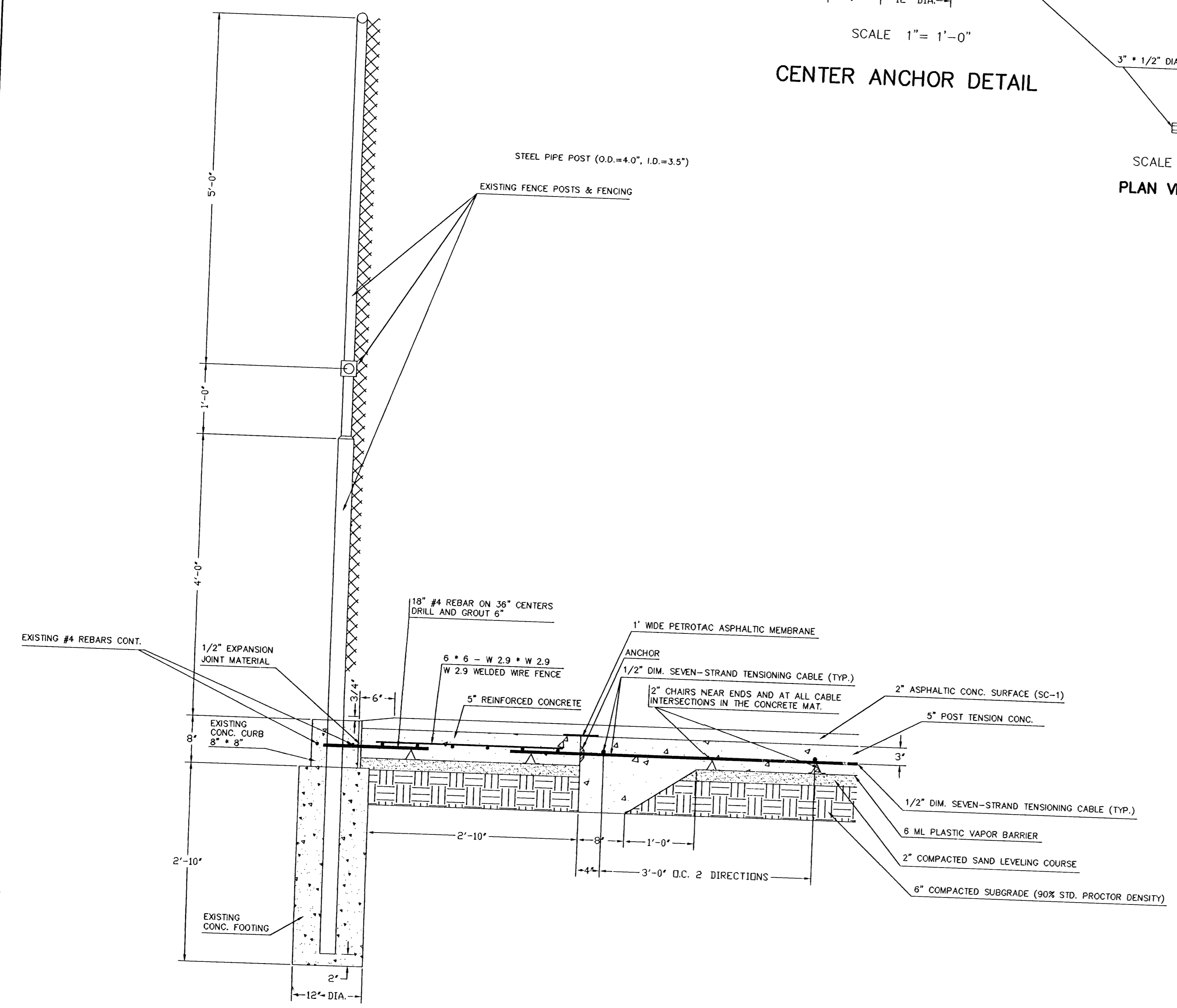
SECTION "A"- "A" SCALE 1" = 1'-0"
