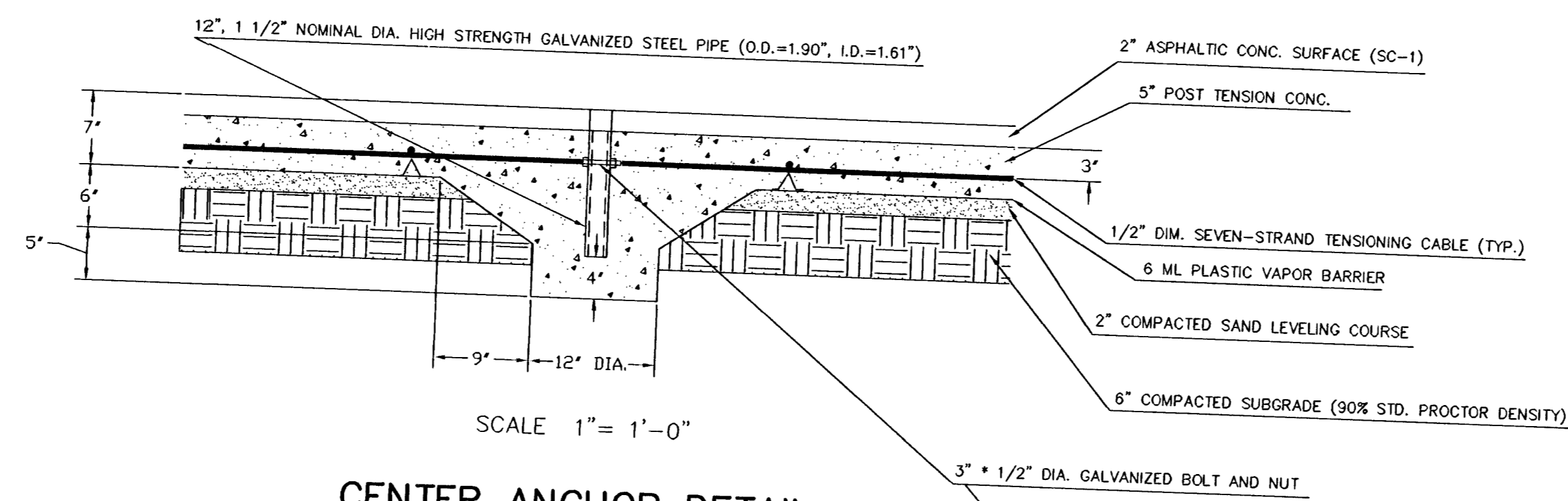
CENTER ANCHOR DETAIL SCALE 1" = 1'-0"
