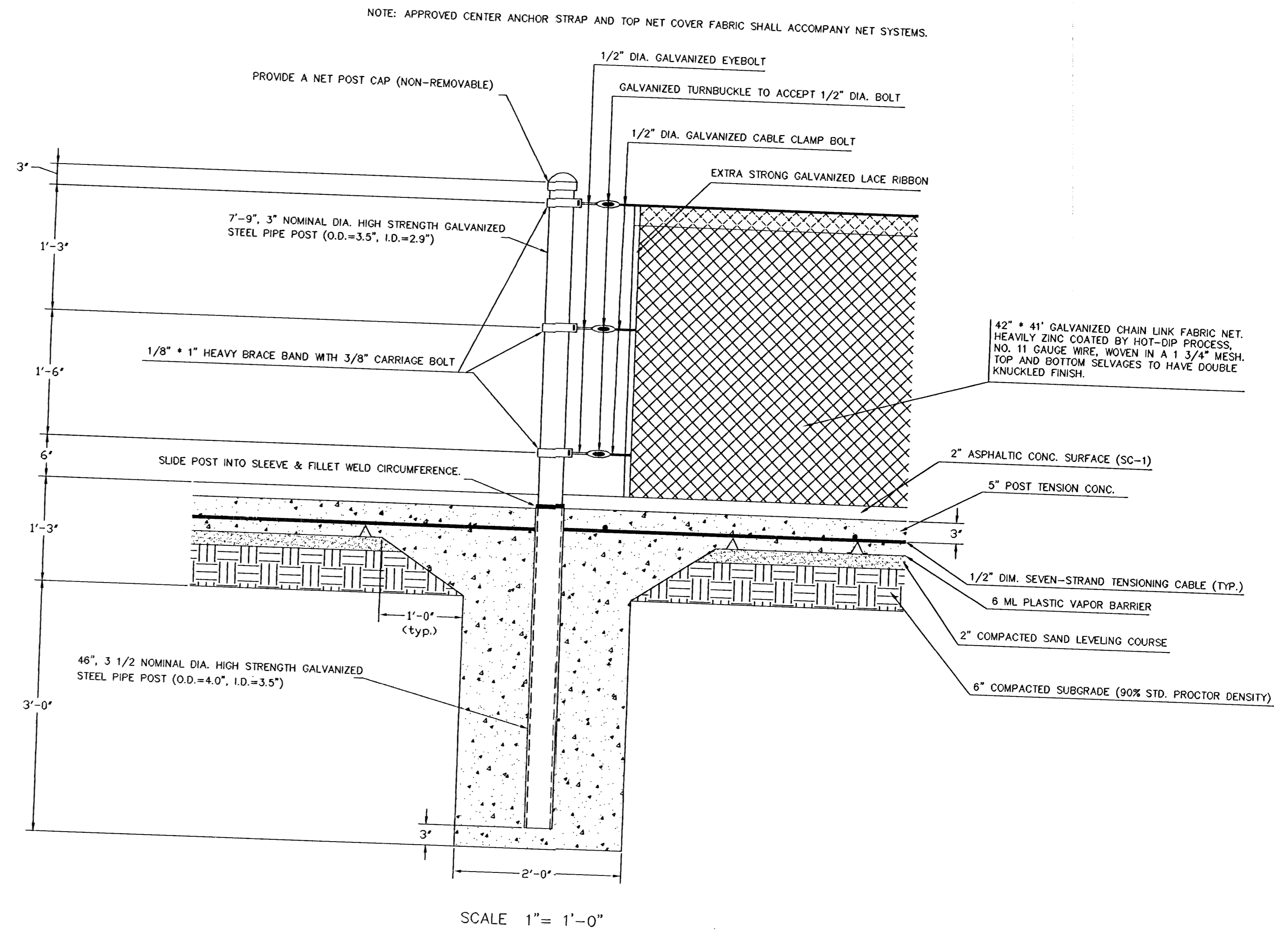
NET & NET POST DETAIL SCALE 1" = 1'-0"
