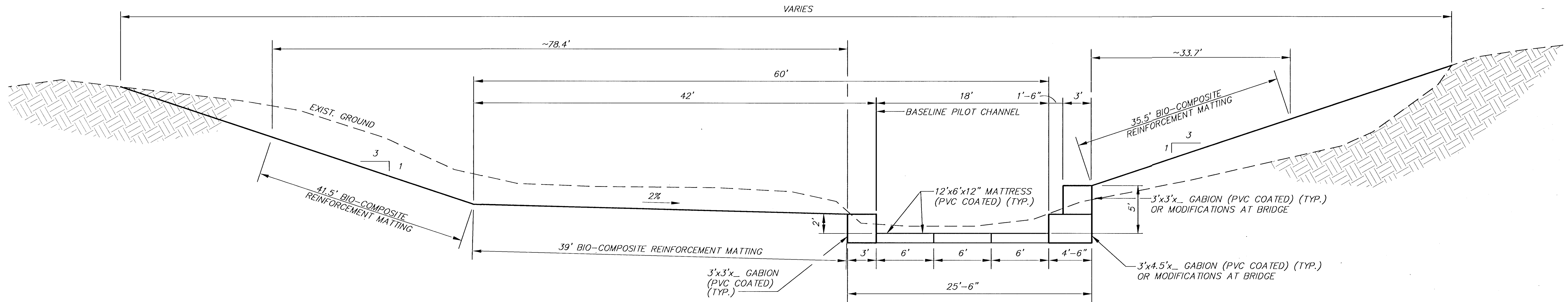
TYPICAL CANAL SECTION (LOOKING DOWNSTREAM)
