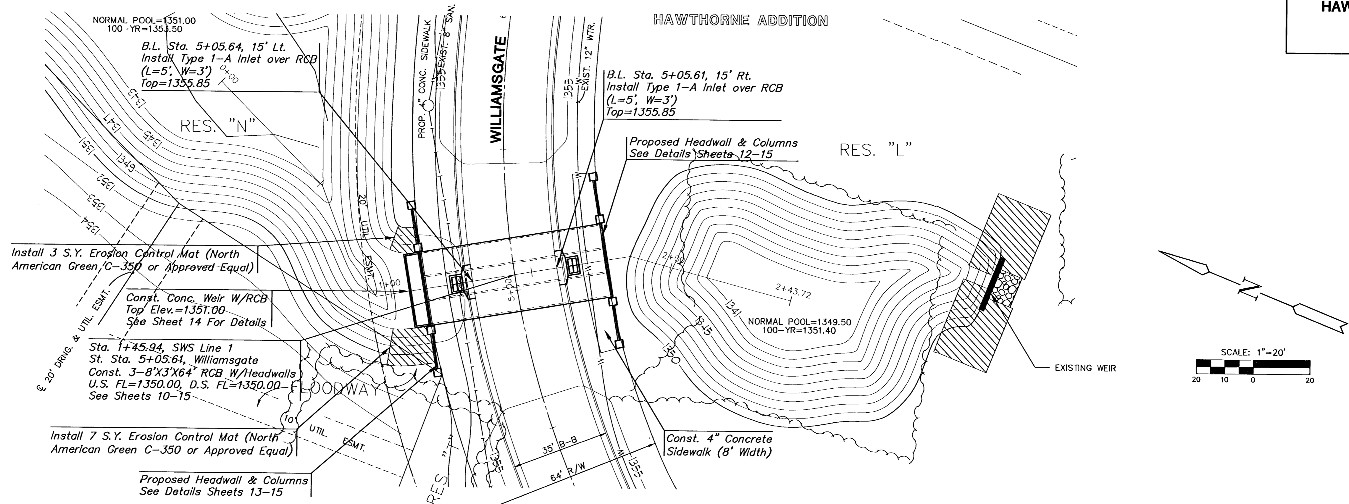
PLAN LINE 1 SCALE: 1"=20'
