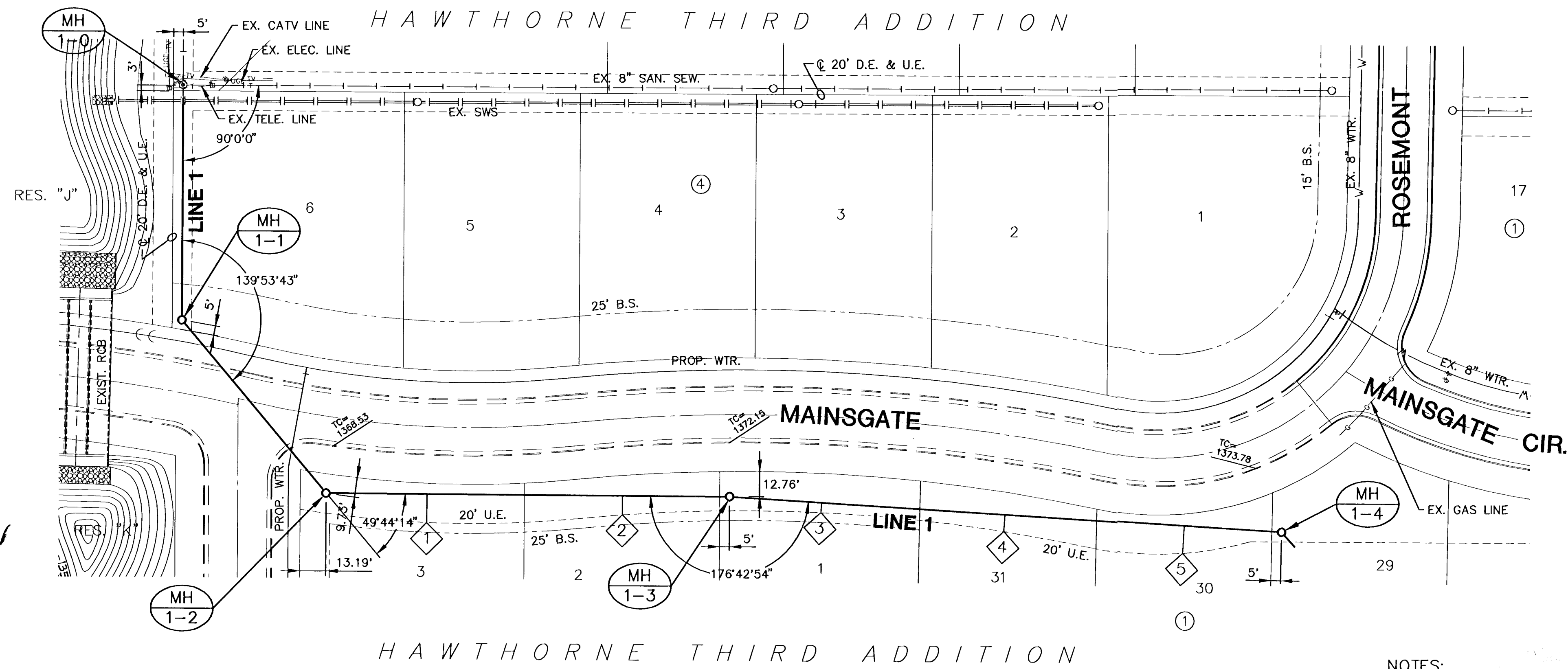
PLAN LINE 1 SCALE: 1"=40'
