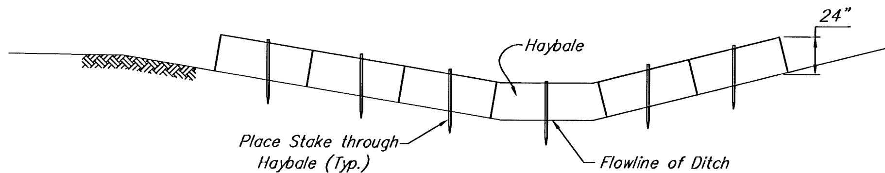
HAY BALE DITCH CHECK
