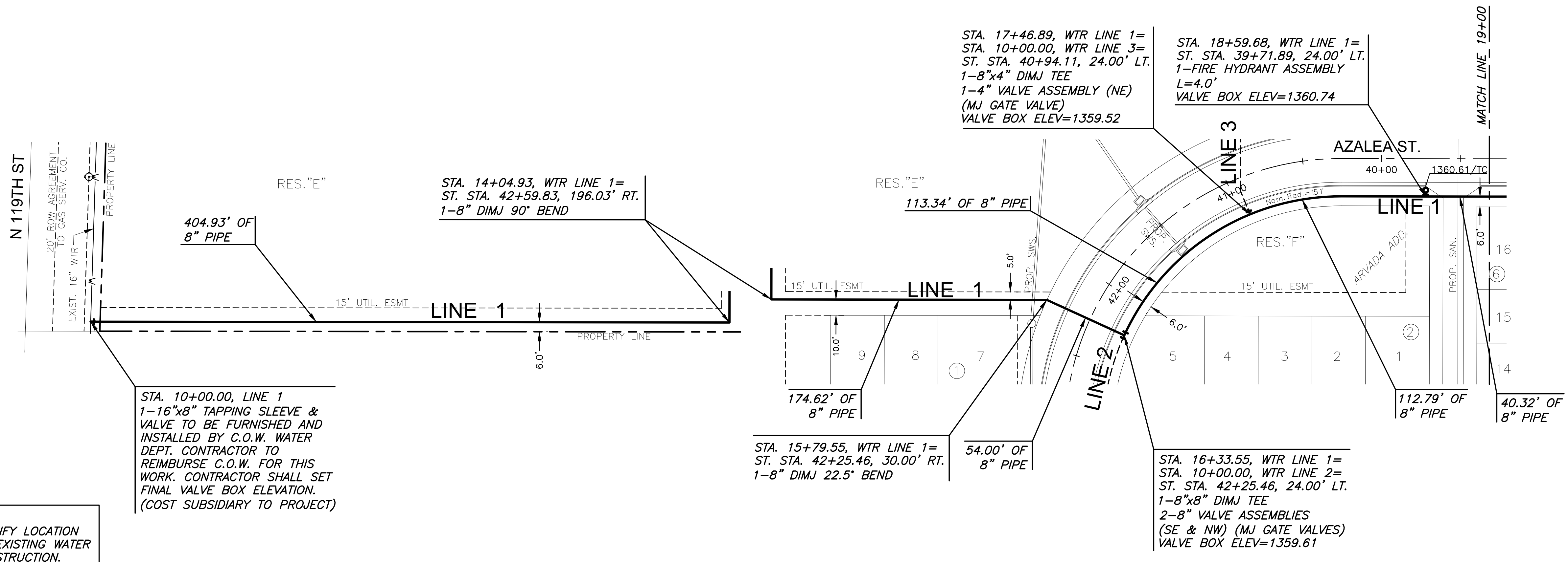
PLAN WTR LINE 1 PROFILE WTR LINE 1
