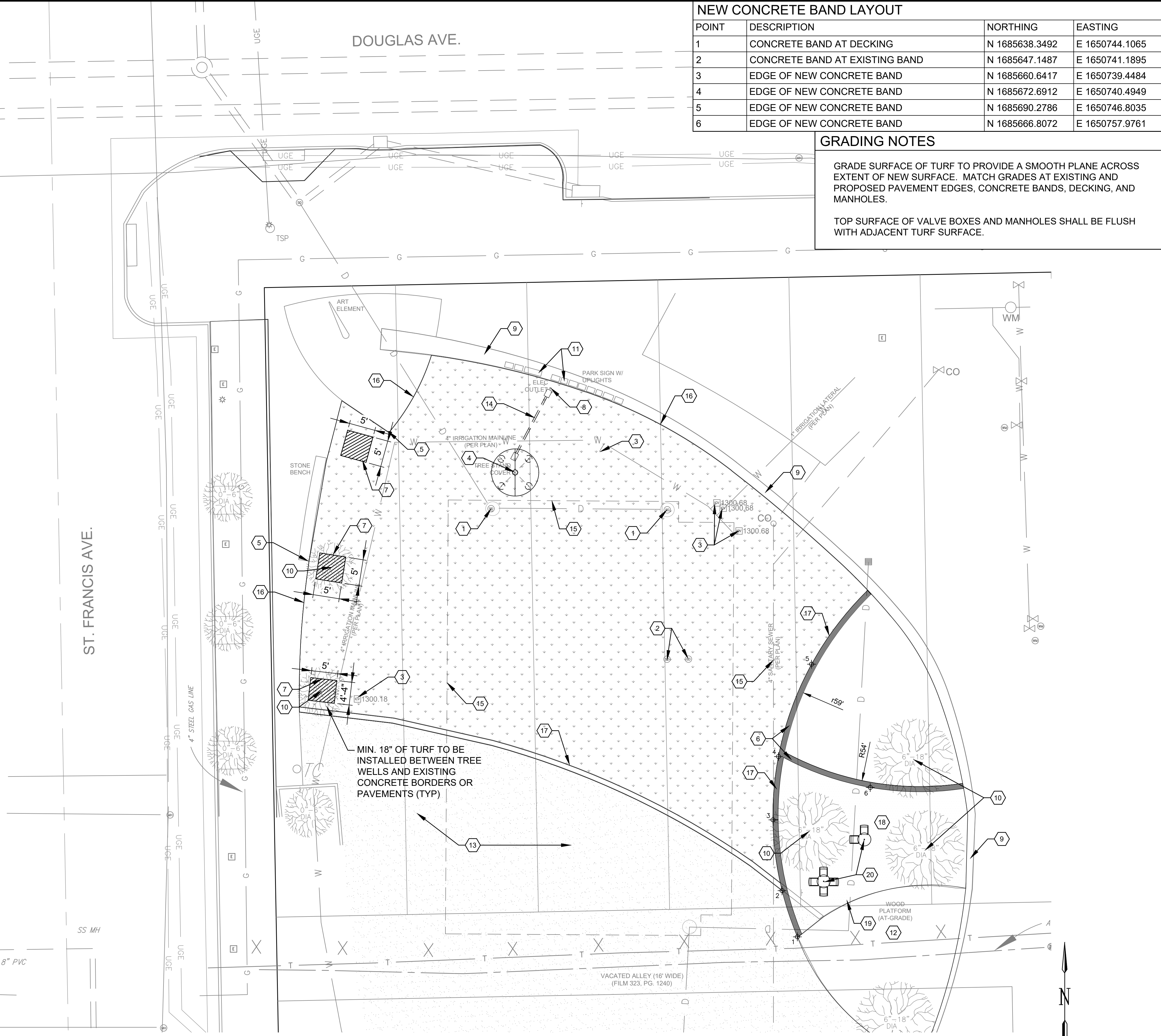
1 LAYOUT PLAN SCALE: 1" = 10'
