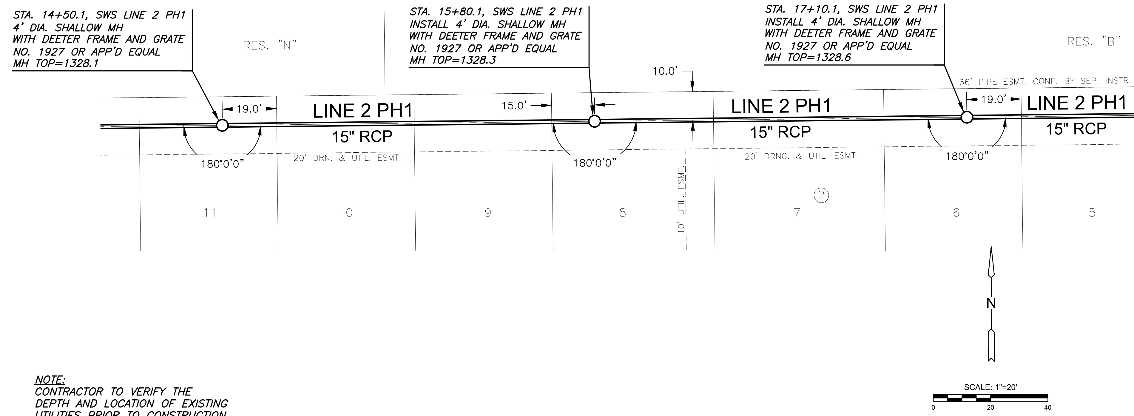
PLAN SWS LINE 2 PH1 (CONT. 1) PROFILE SWS LINE 2 PH1 (CONT. 1)
