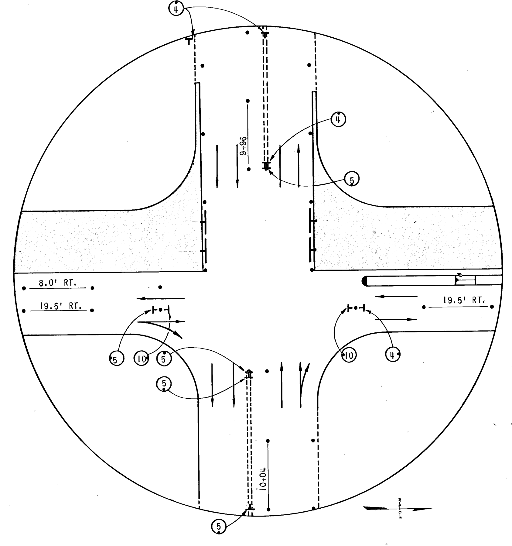
INTERSECTION DETAIL NOT TO SCALE
