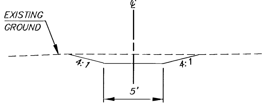
TYPICAL DITCH CROSS SECTION
