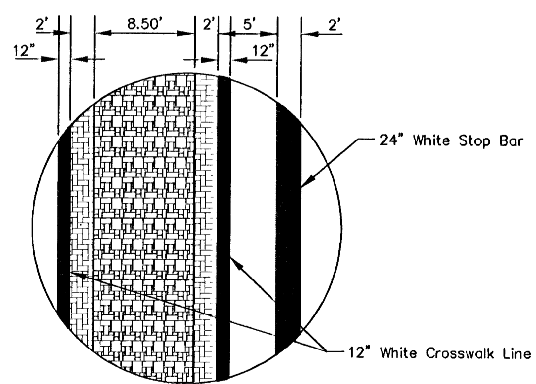
Crosswalk Detail
