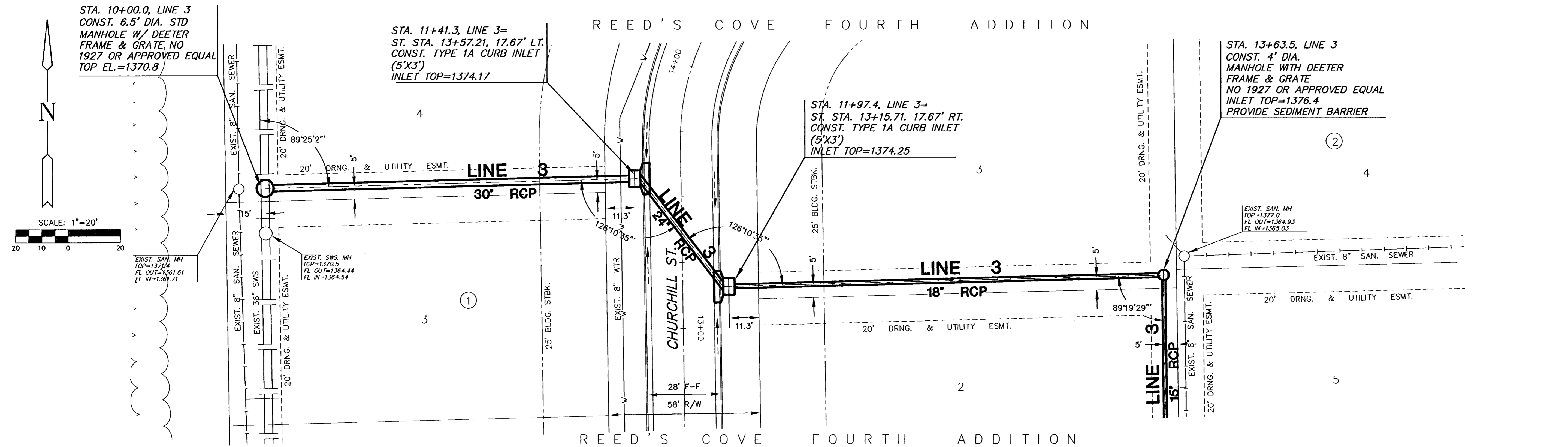
PLAN LINE 3
