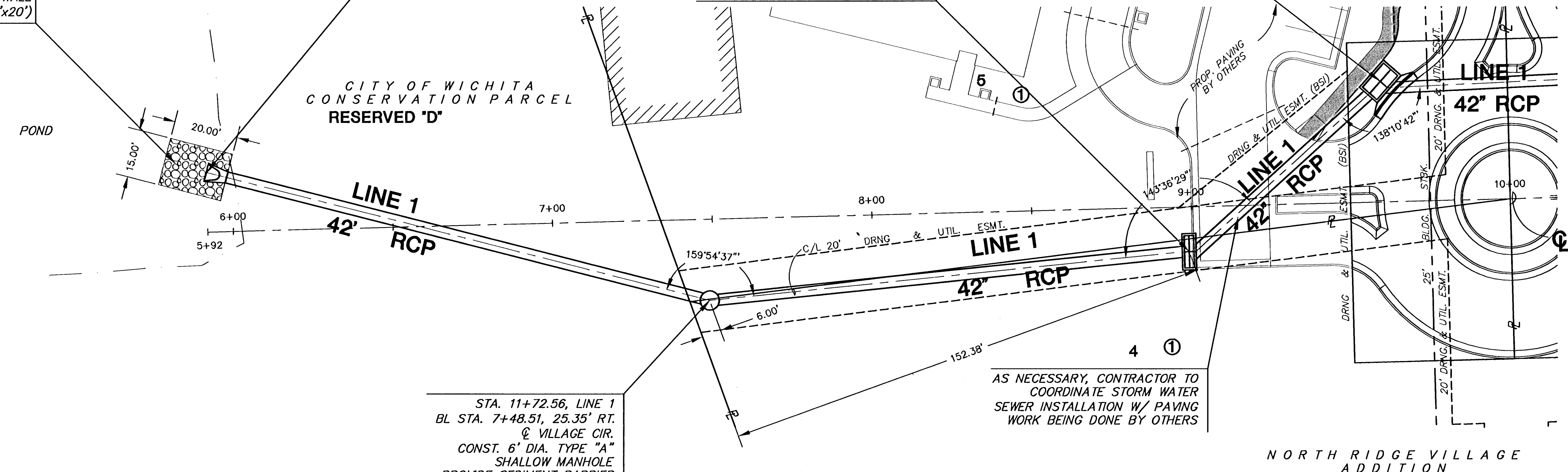
PLAN LINE 1 SCALE: 1"=20'
