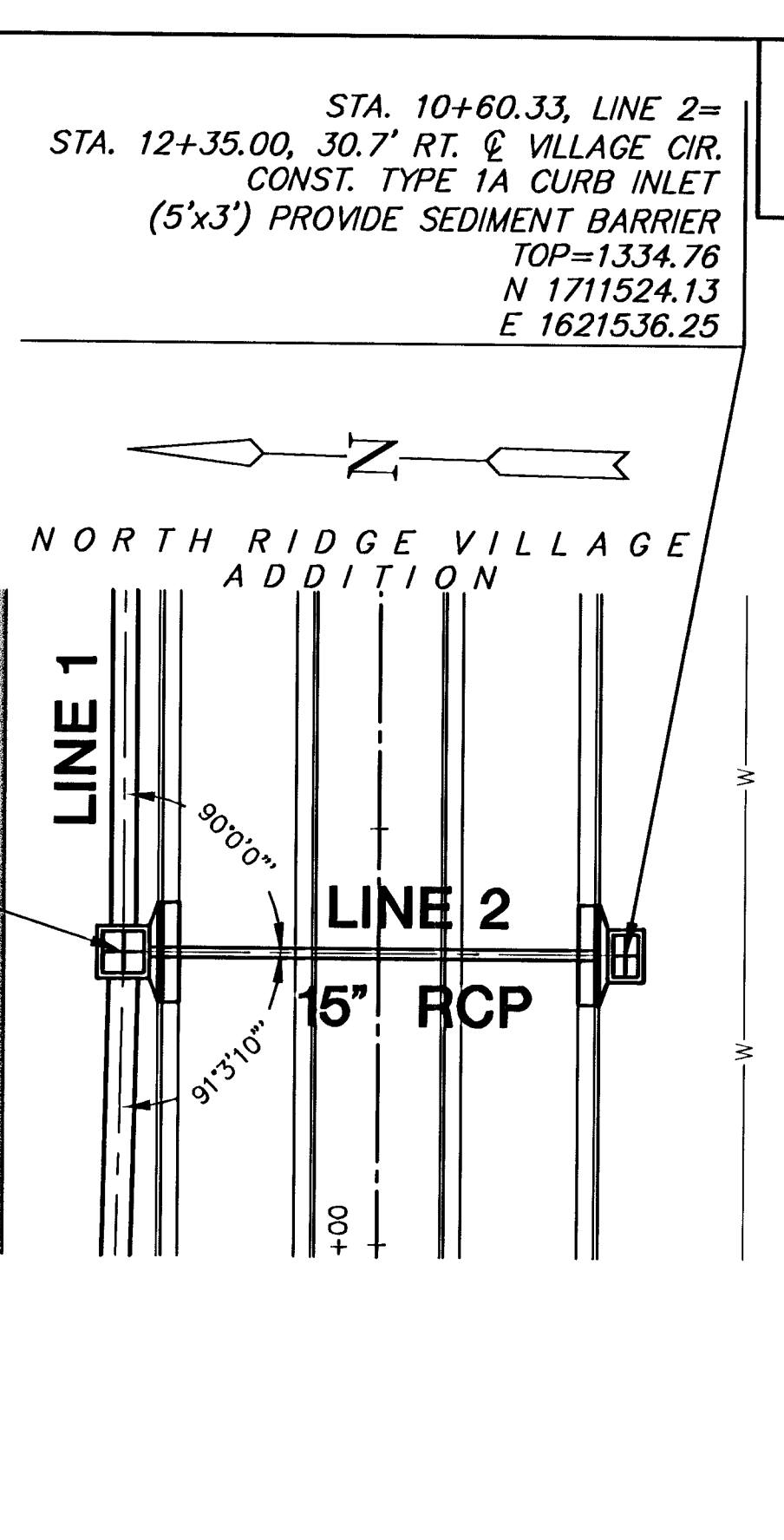
PLAN LINE 2 SCALE: 1"=20'
