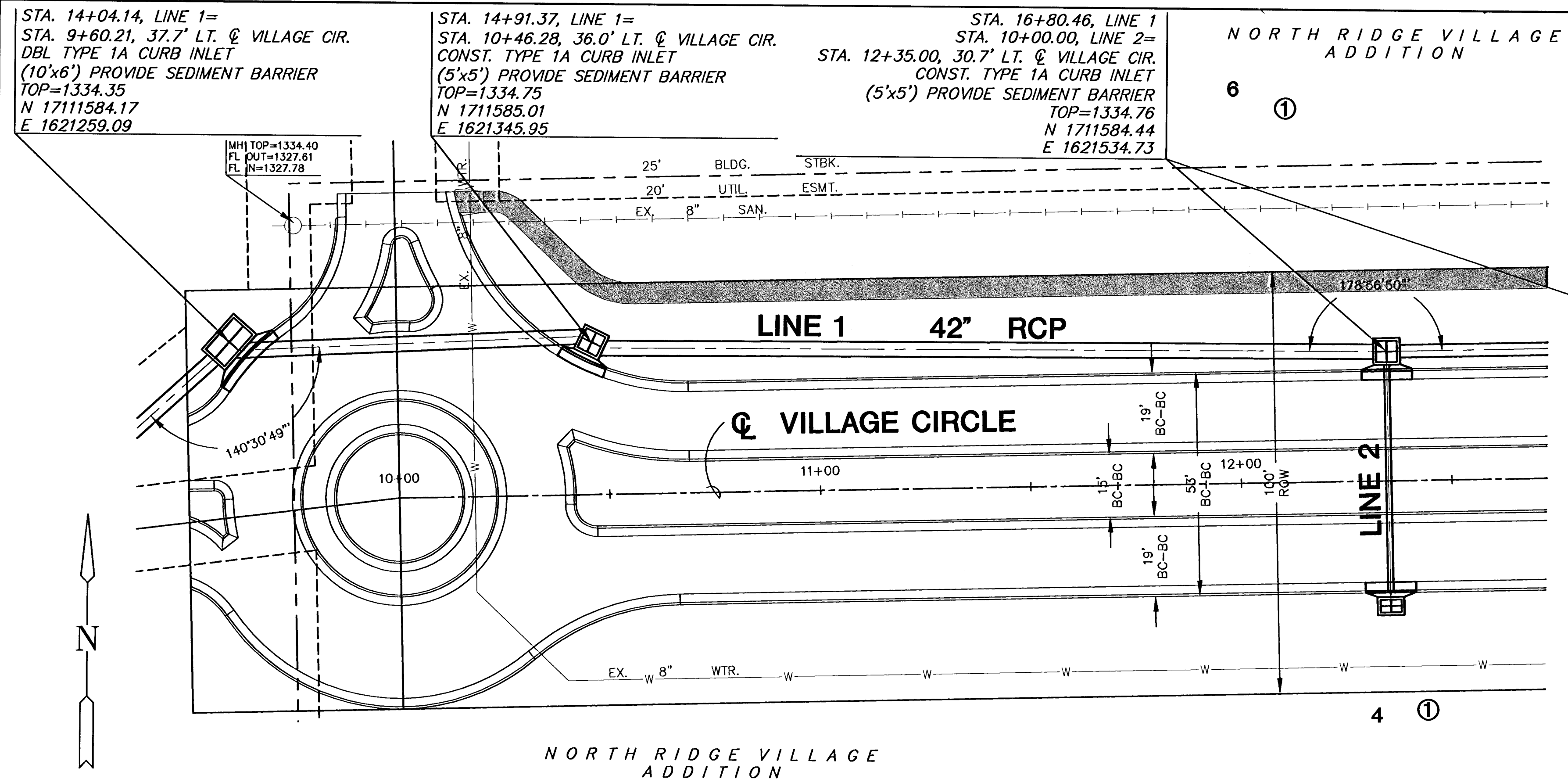
CONT. PLAN LINE 1 SCALE: 1"=20'
