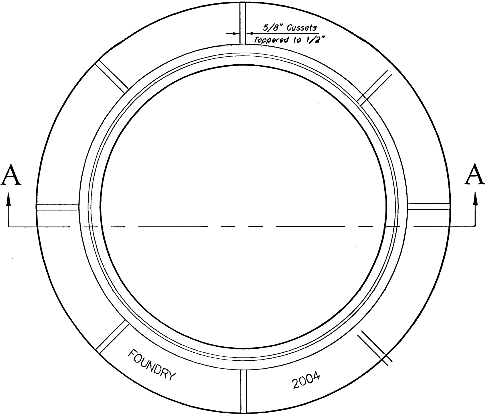
TOP VIEW
