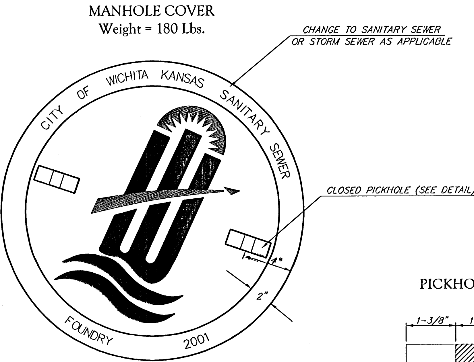
TOP VIEW
