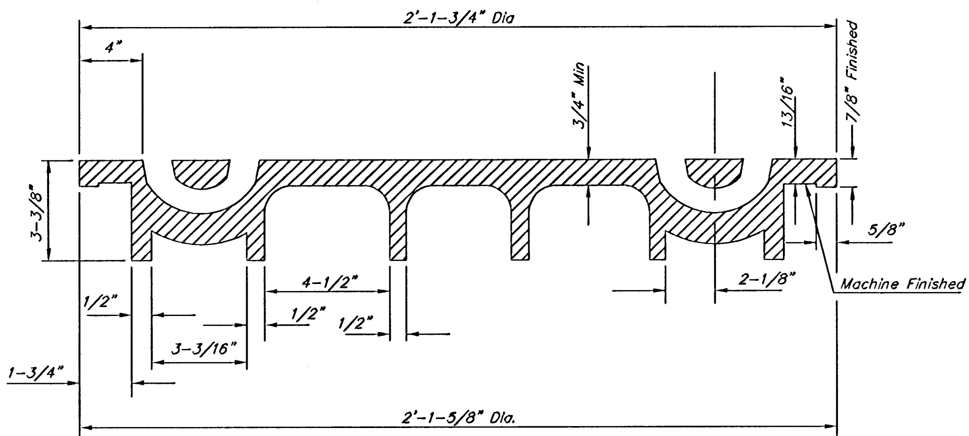
SECTION VIEW
