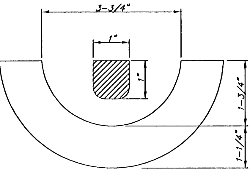
SECTION VIEW
