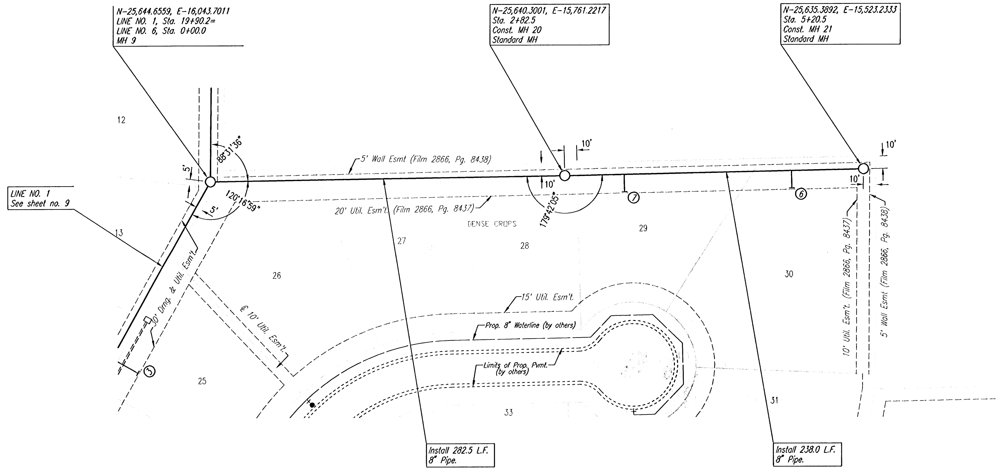
SANITARY SEWER LINE NO. 6
