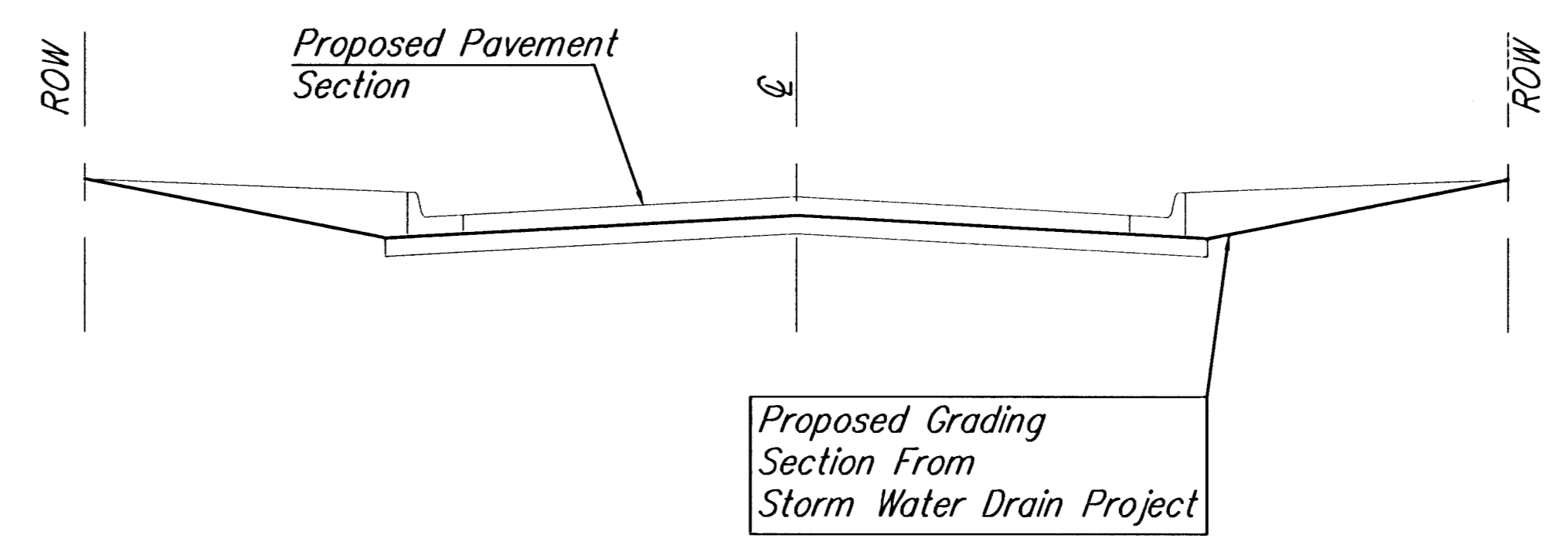
ROW GRADING DETAIL
