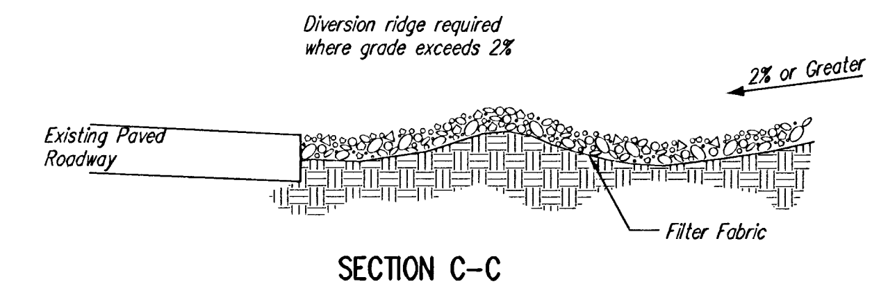
SECTION C-C
