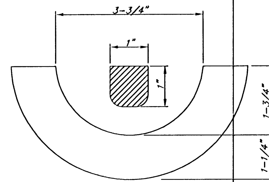
SECTION VIEW
