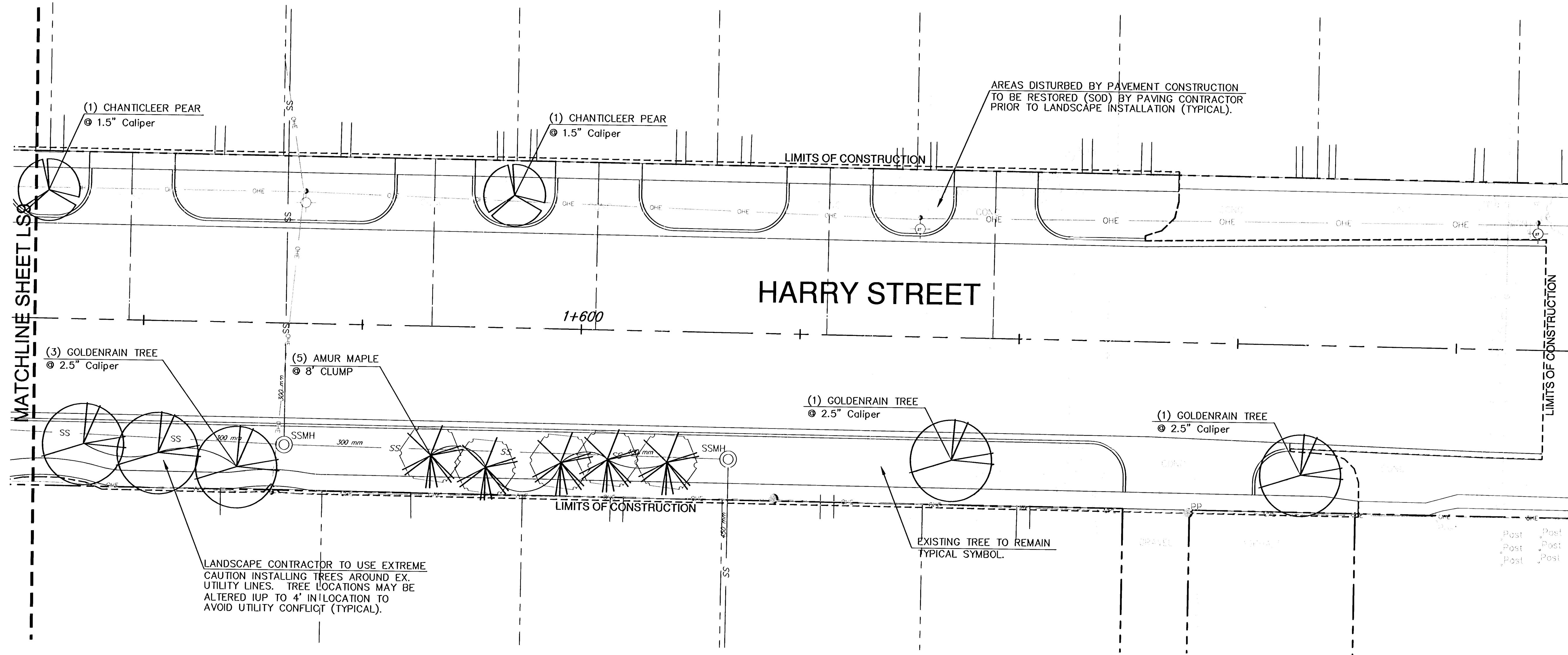
STREET PLANTING PLAN SCALE: 1:200
