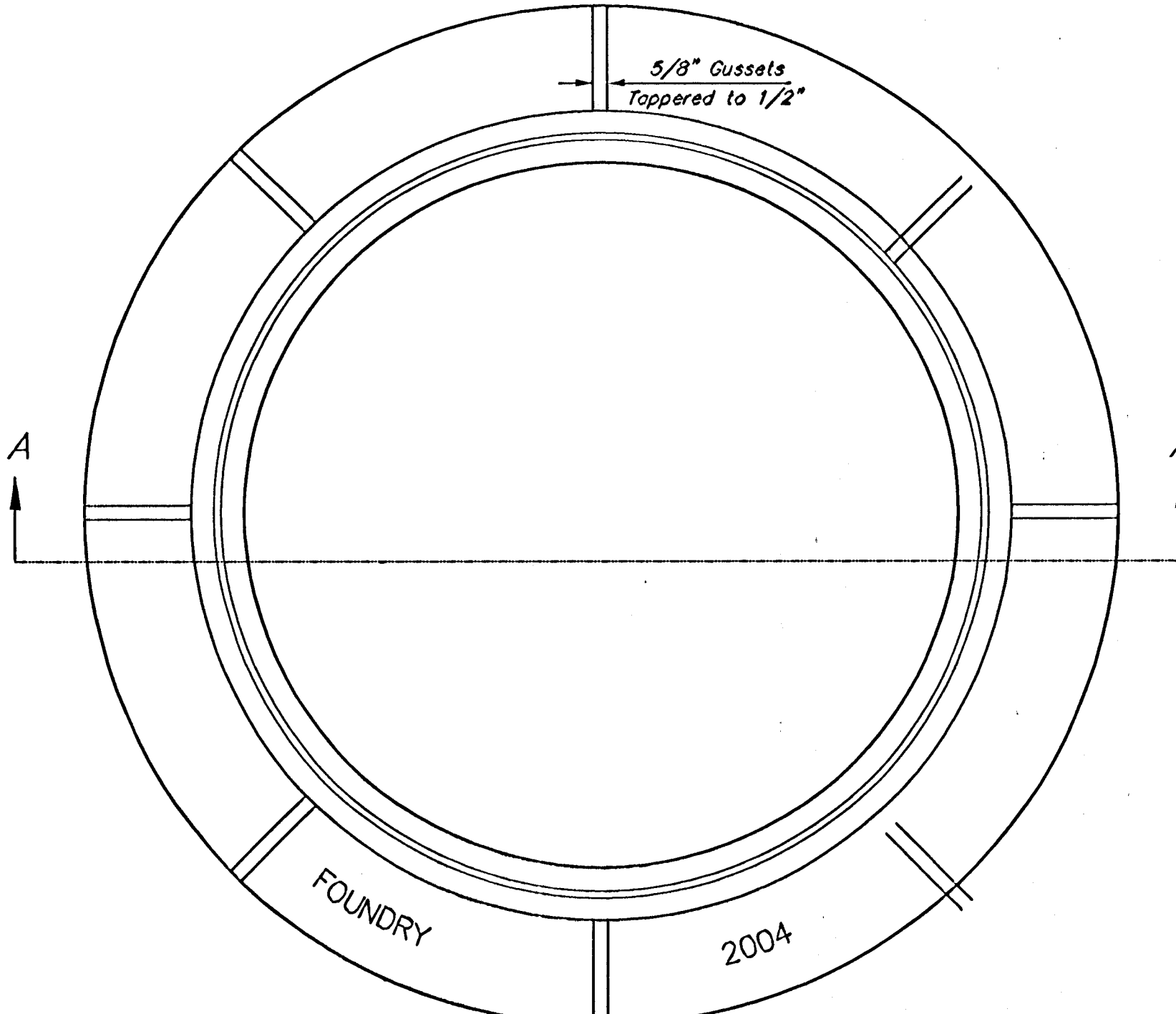
TOP VIEW
