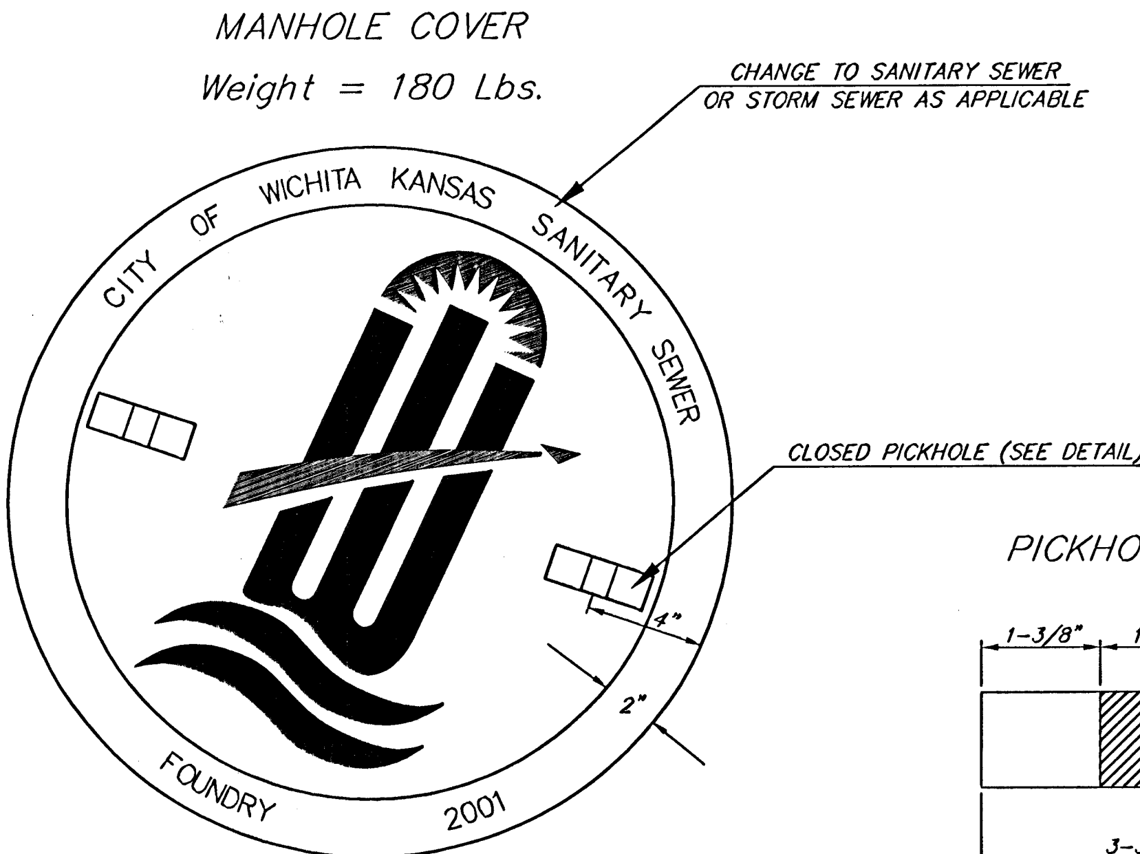
TOP VIEW
