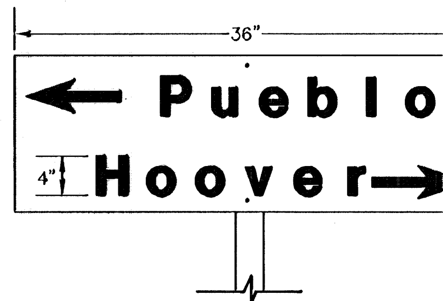
FLAT PLATE STREET NAME SIGN
