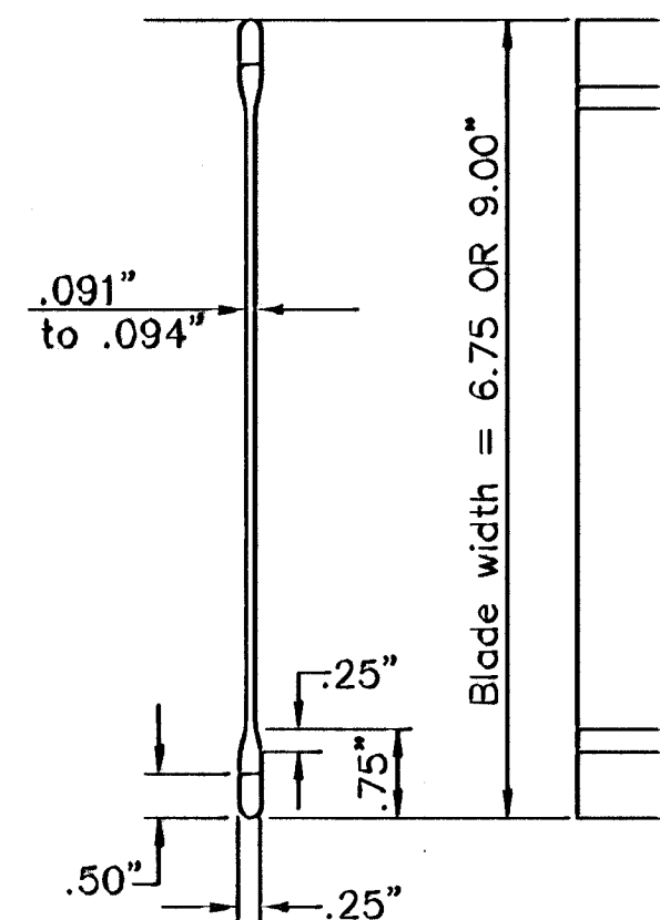
STREET NAME S BLADE DETAILS
