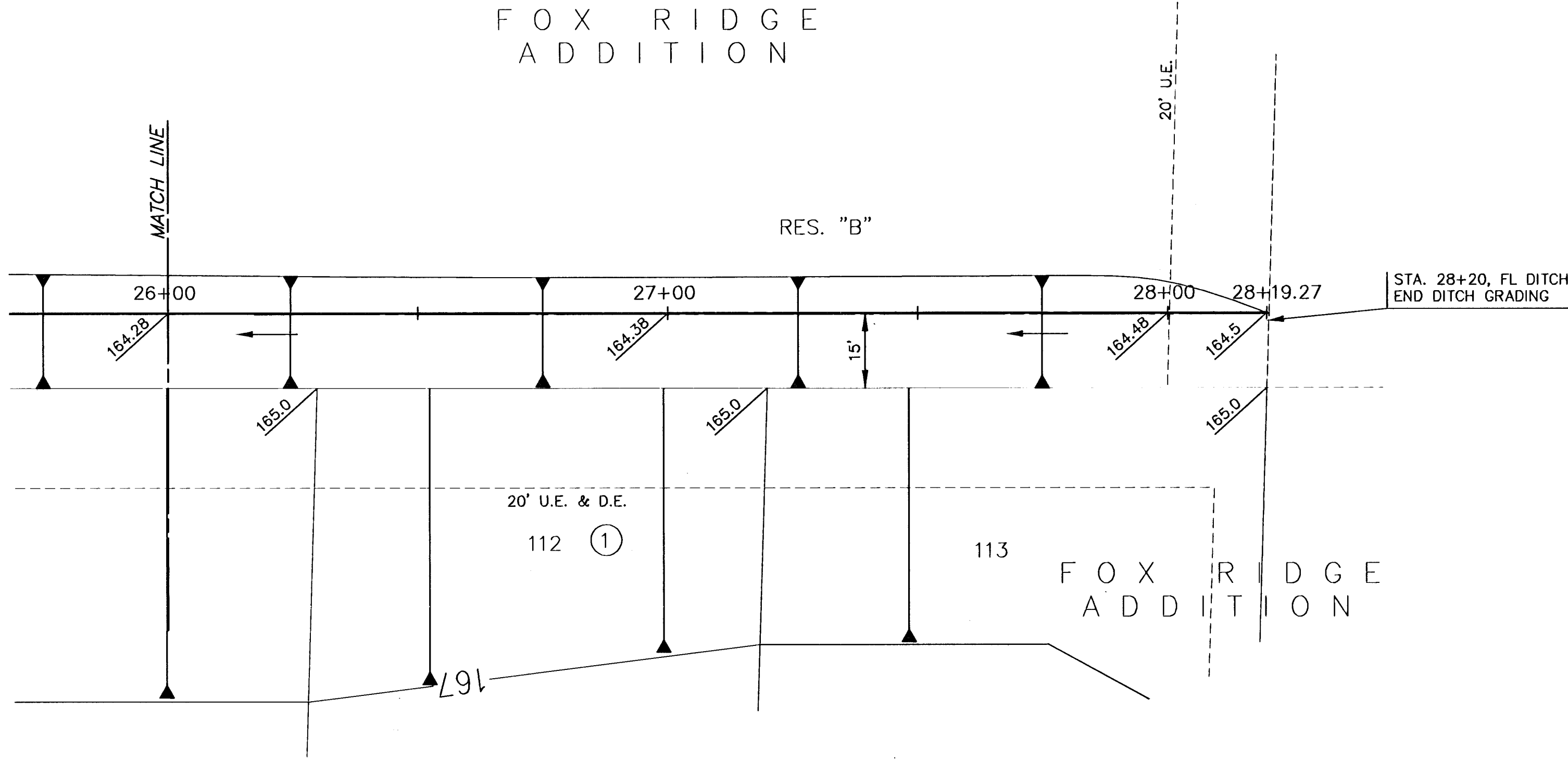
PLAN DITCH GRADING
