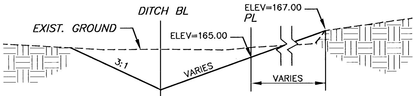
TYPICAL DITCH SECTION
