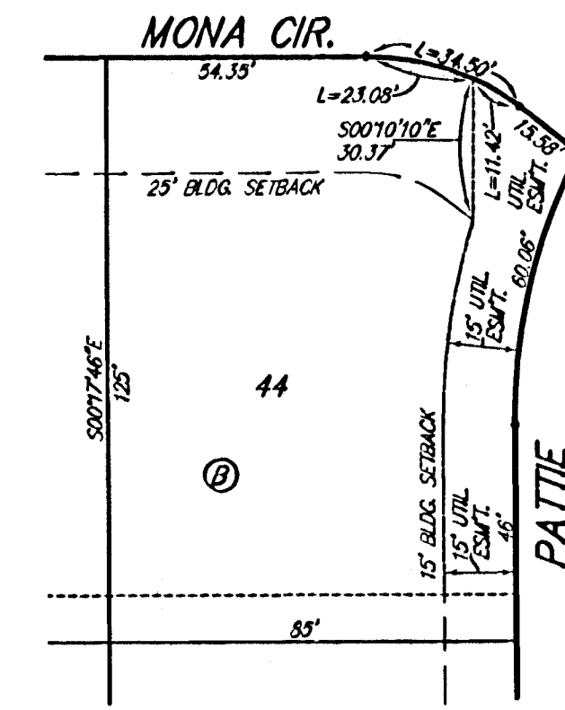
DETAIL "B" (NO SCALE)
