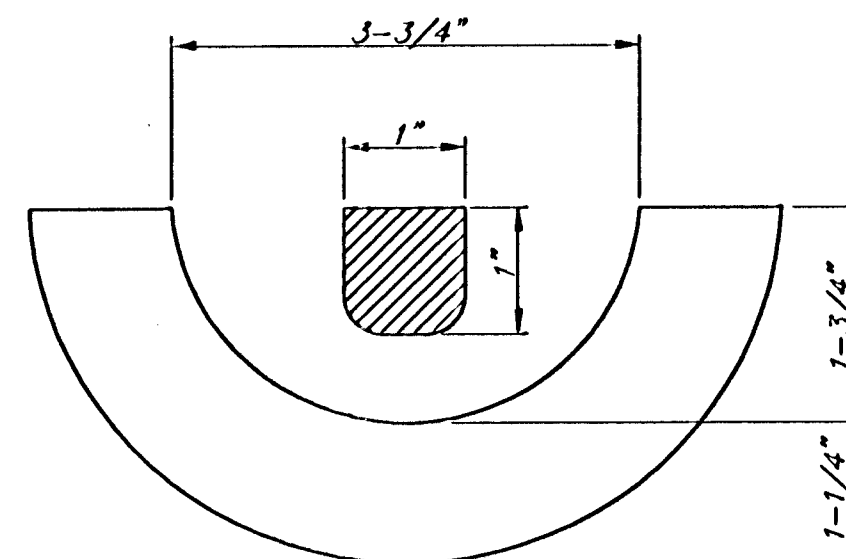
SECTION VIEW
