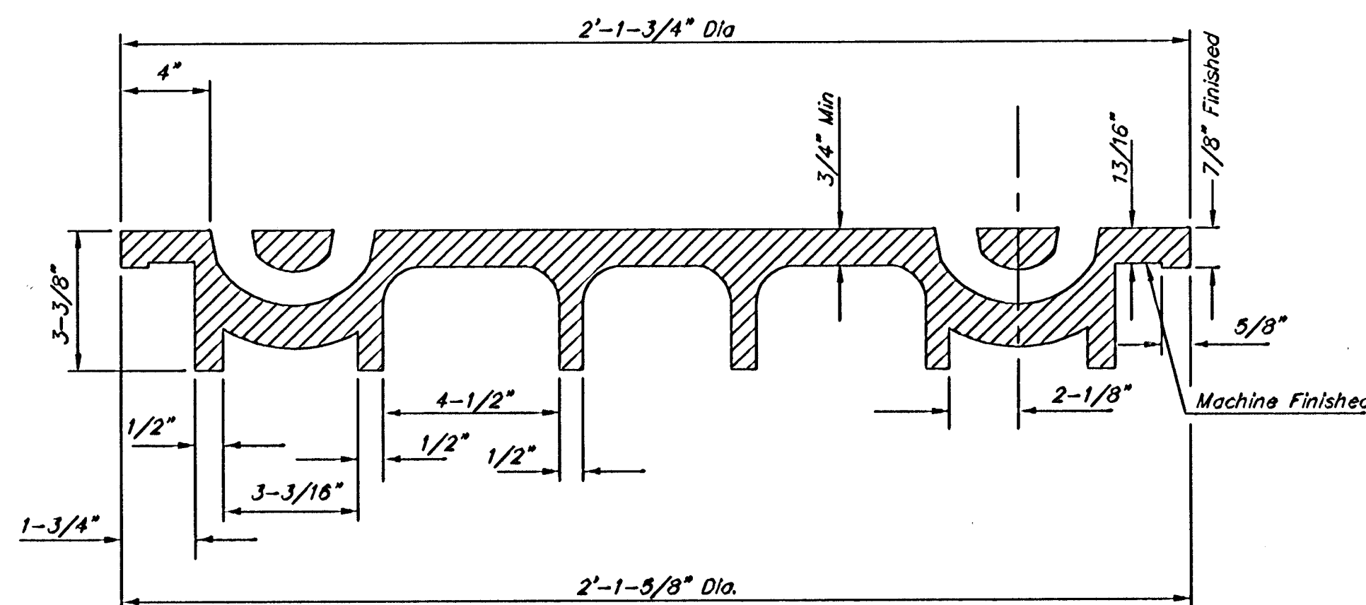
SECTION VIEW
