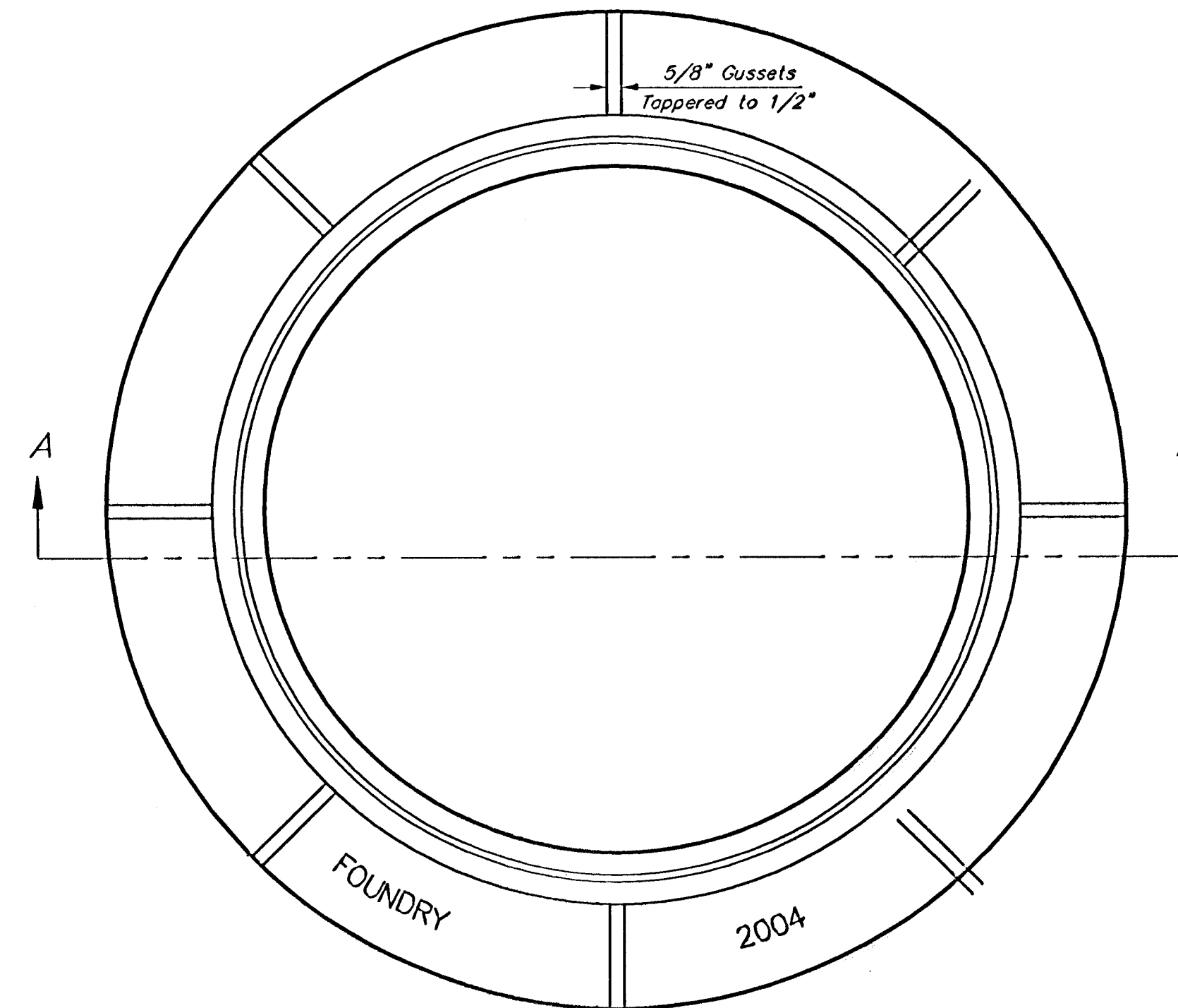
TOP VIEW
