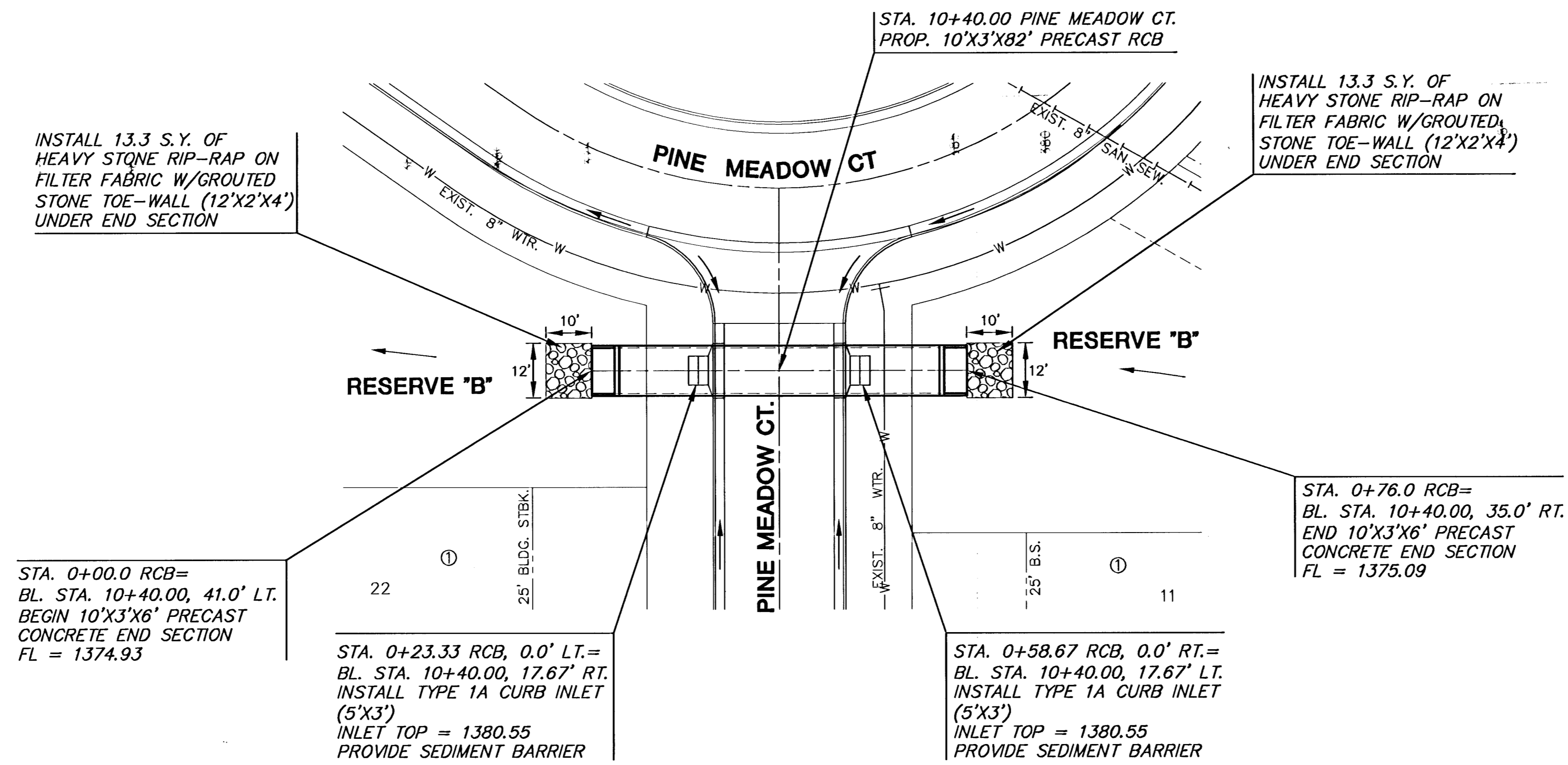
PLAN RCB SCALE: 1"=20'
