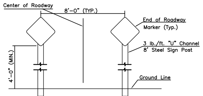
TYPICAL END OF ROADWAY SIGN MOUNTING INSTALLATION
