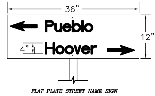
FLAT PLATE STREET NAME SIGN
