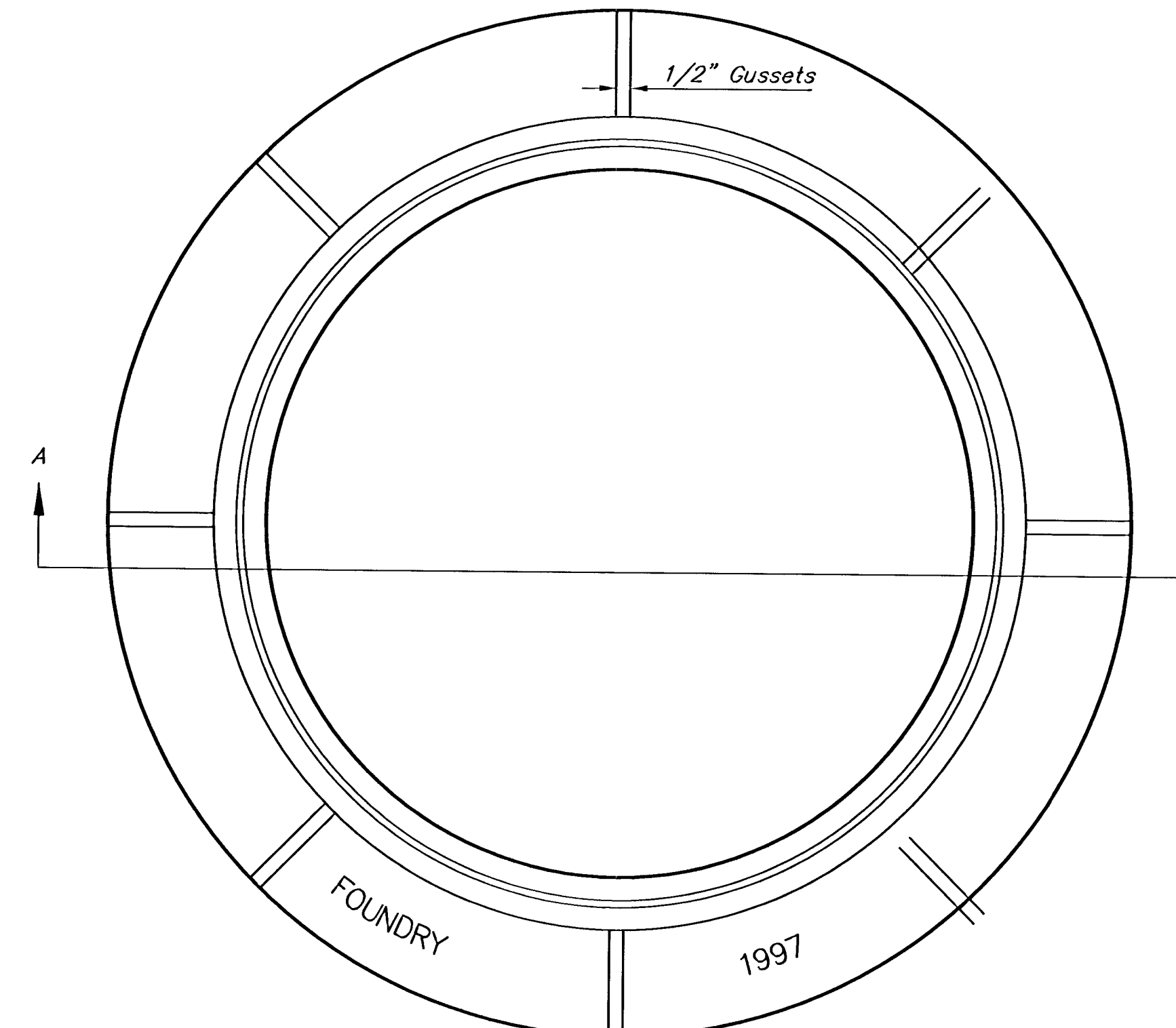
TOP VIEW
