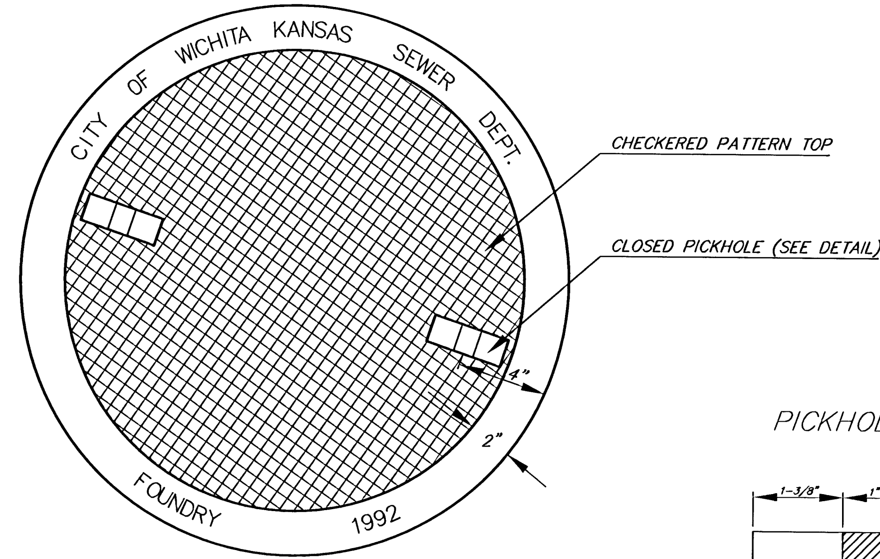
TOP VIEW
