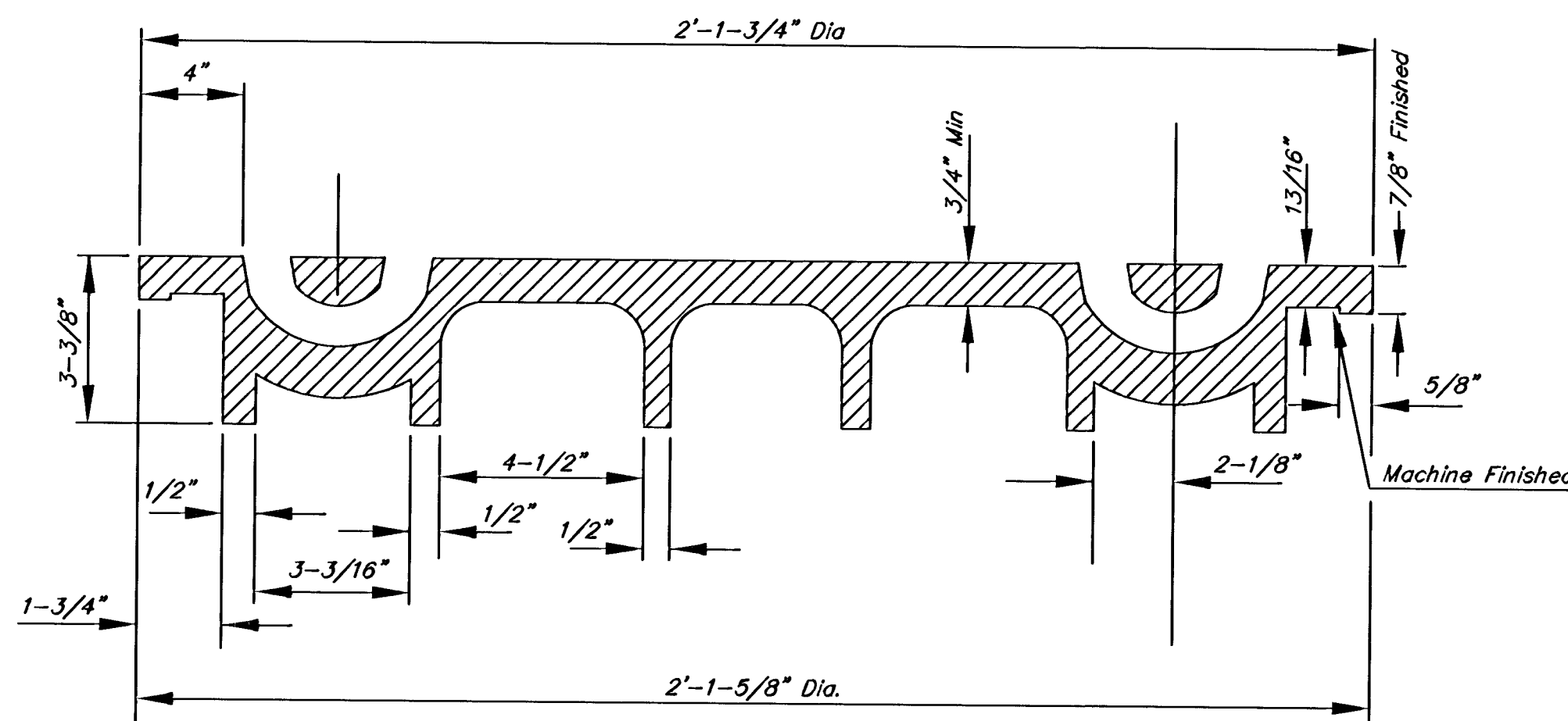
SECTION VIEW
