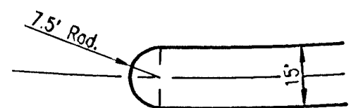
TYPICAL MEDIAN RESERVE DETAIL
