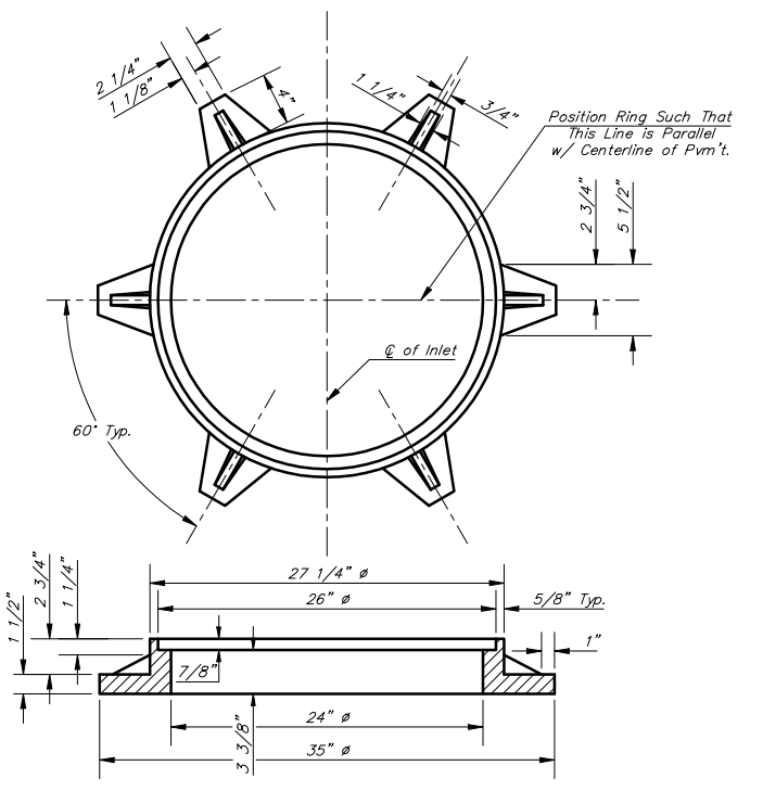
MANHOLE RING AND COVER Weight = 180 lbs.
