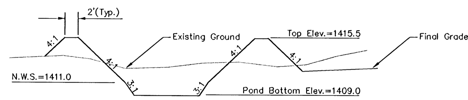
DETENTION POND DETAIL
