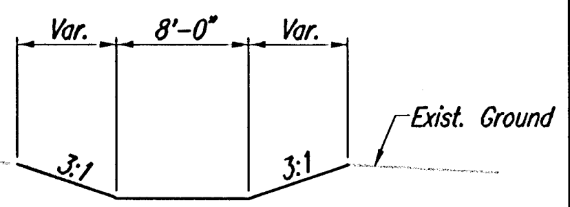
TYPICAL CHANNEL SECTION
