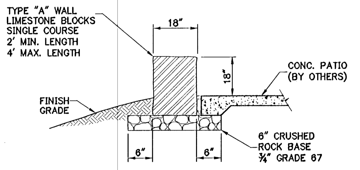
TYPE "A" WALL LIMESTONE BLOCKS SINGLE COURSE 2' MIN. LENGTH 4' MAX. LENGTH PATIO WALL DETAIL SCALE: N.T.S.
