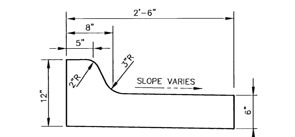
REVERSE CURB & GUTTER
