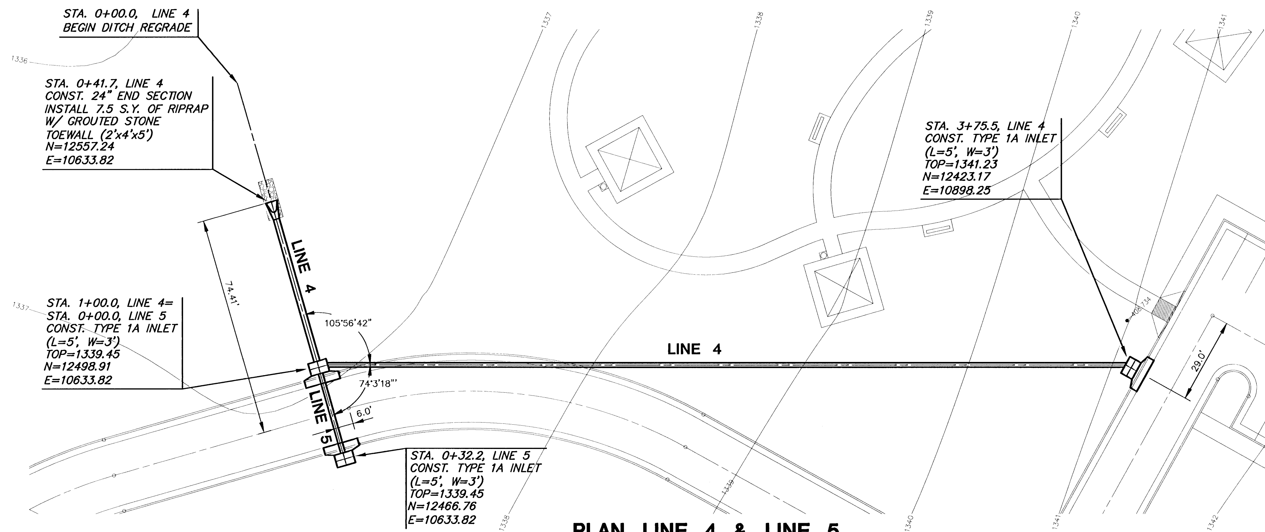
PLAN LINE 4 & LINE 5
