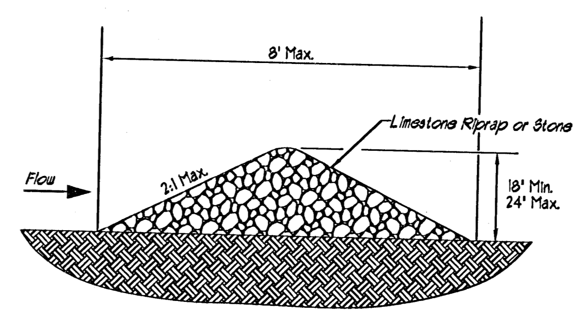
DETAIL OF ROCK DITCH CHECK INSTALLATION
