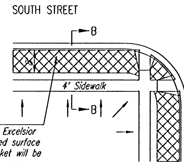
BACK OF CURB PROTECTION DETAIL
