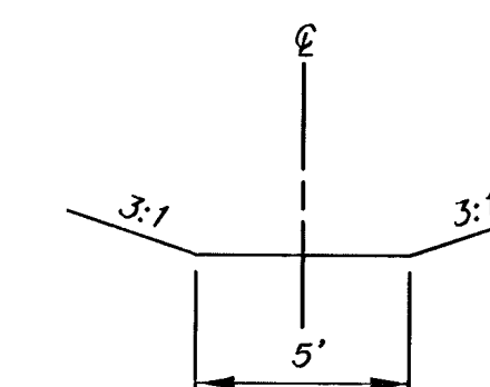
TYPICAL DITCH CROSS SECTION
