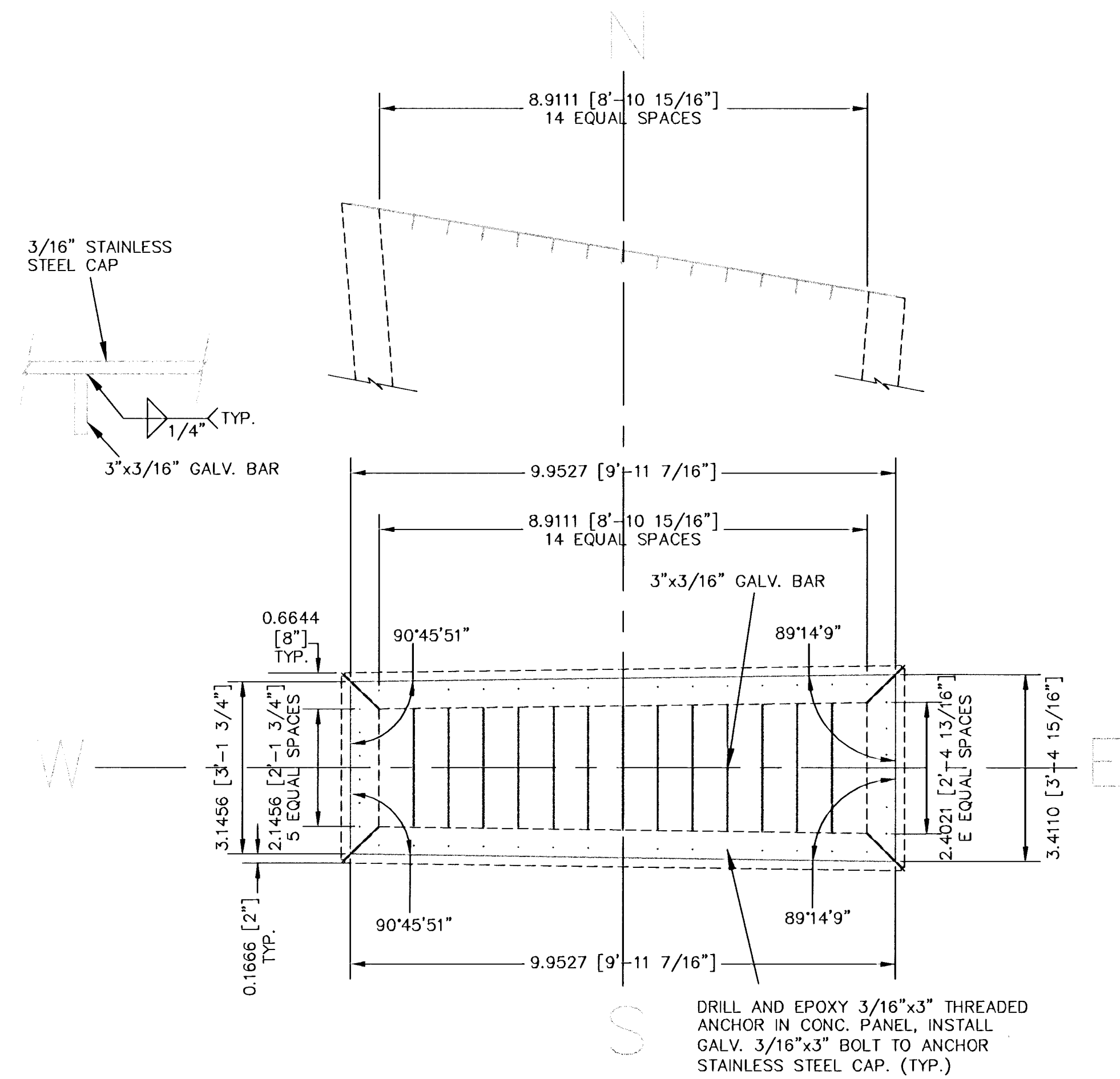
TOWER BASE DETAIL SCALE: 1/2"=1'
