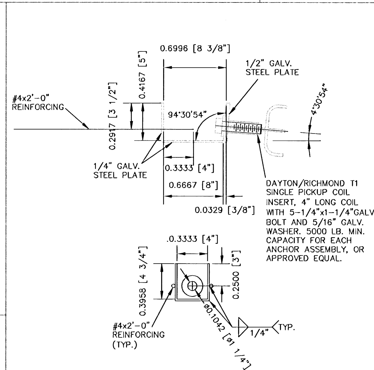
EAST-WEST ANCHOR BOLT ASSEMBLY DETAIL NO SCALE
