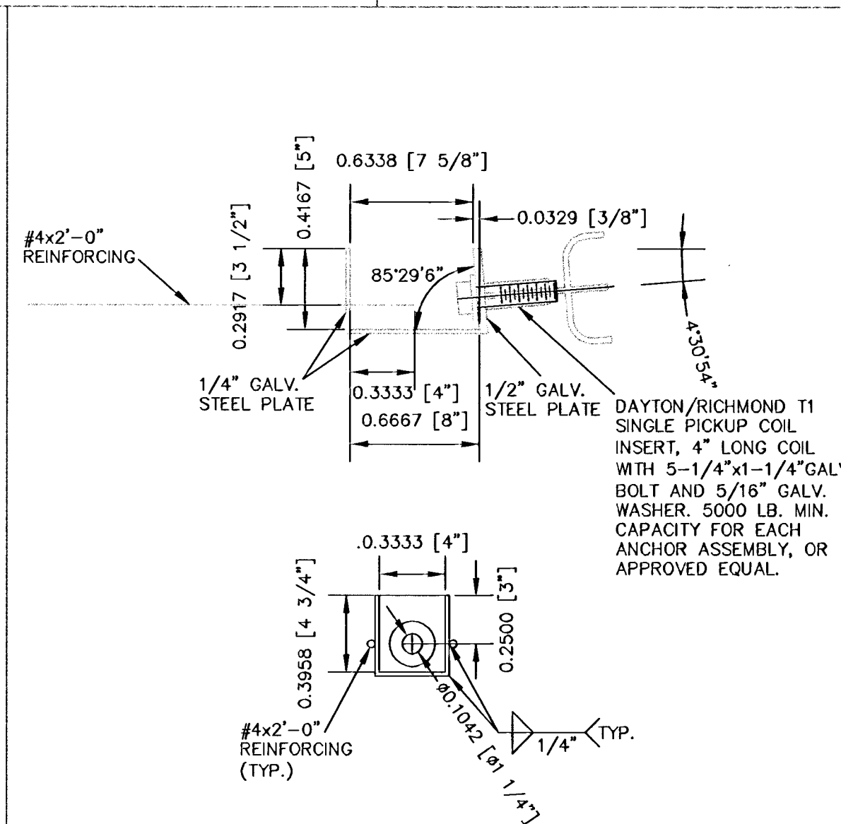
NORTH-SOUTH ANCHOR BOLT ASSEMBLY DETAIL NO SCALE
