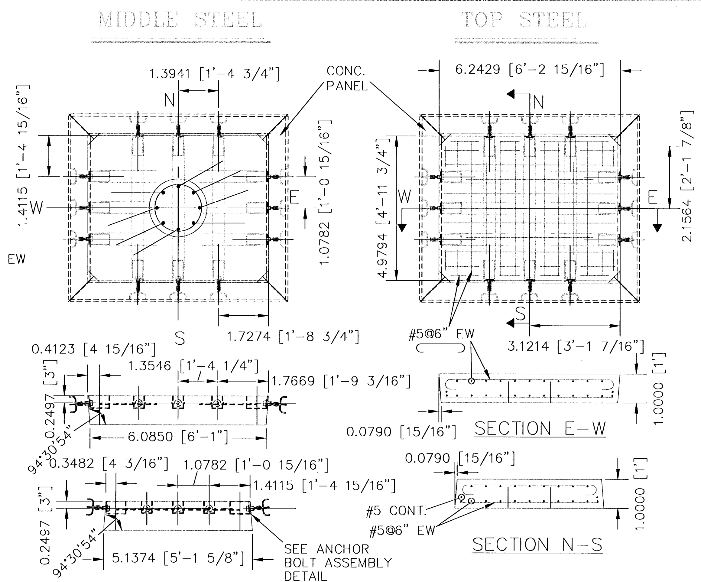
CONNECTOR HEAD DETAIL SCALE: 1/2"=1'
