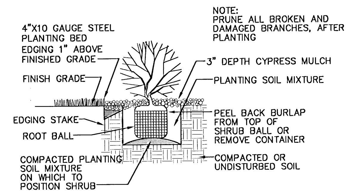
3 SHRUB PLANTING DETAIL LP-1 NOT TO SCALE
