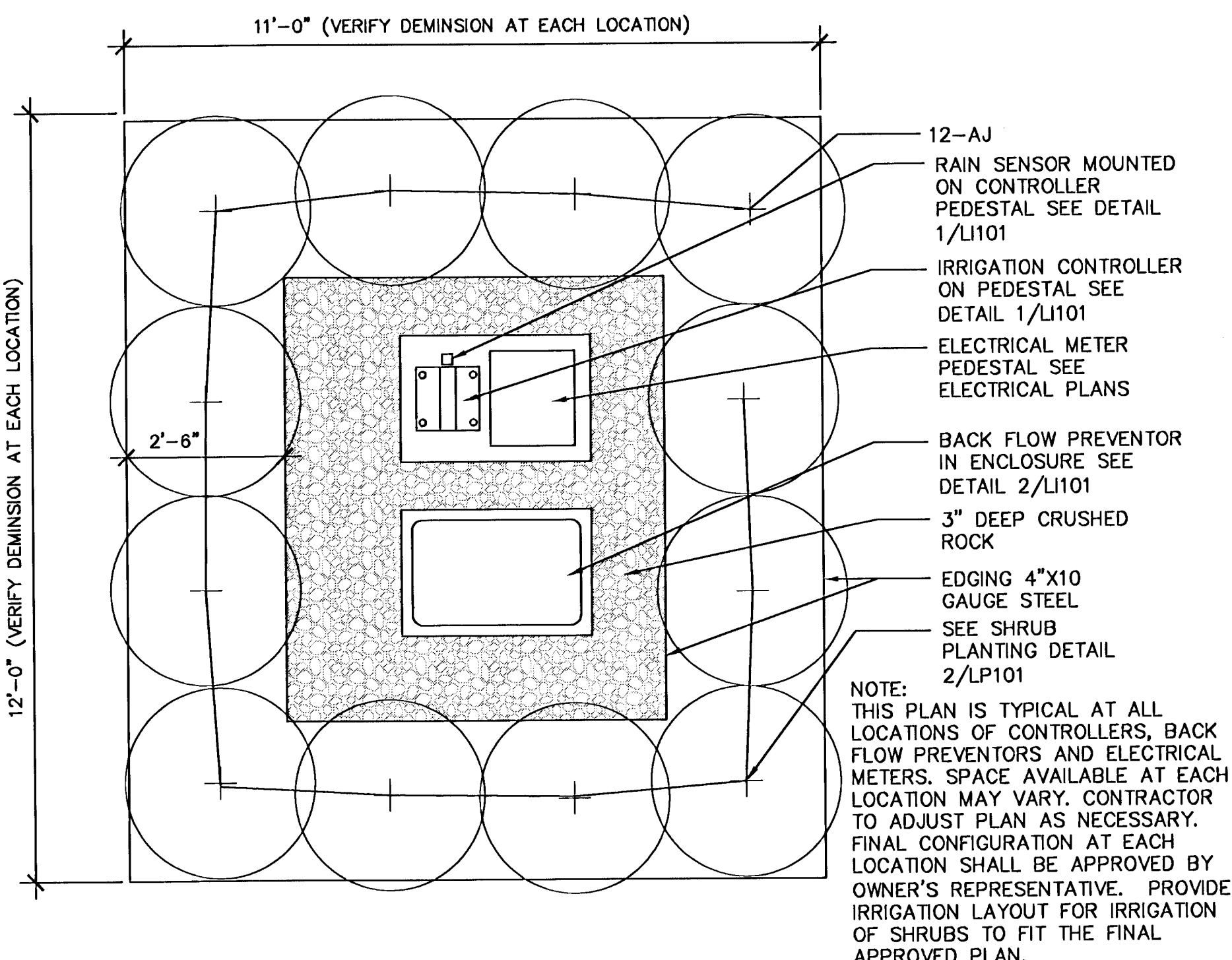
2 TYP. PLANTING AT CONTROLLER & BACKFLOW PREVENTOR LP-1 NOT TO SCALE
