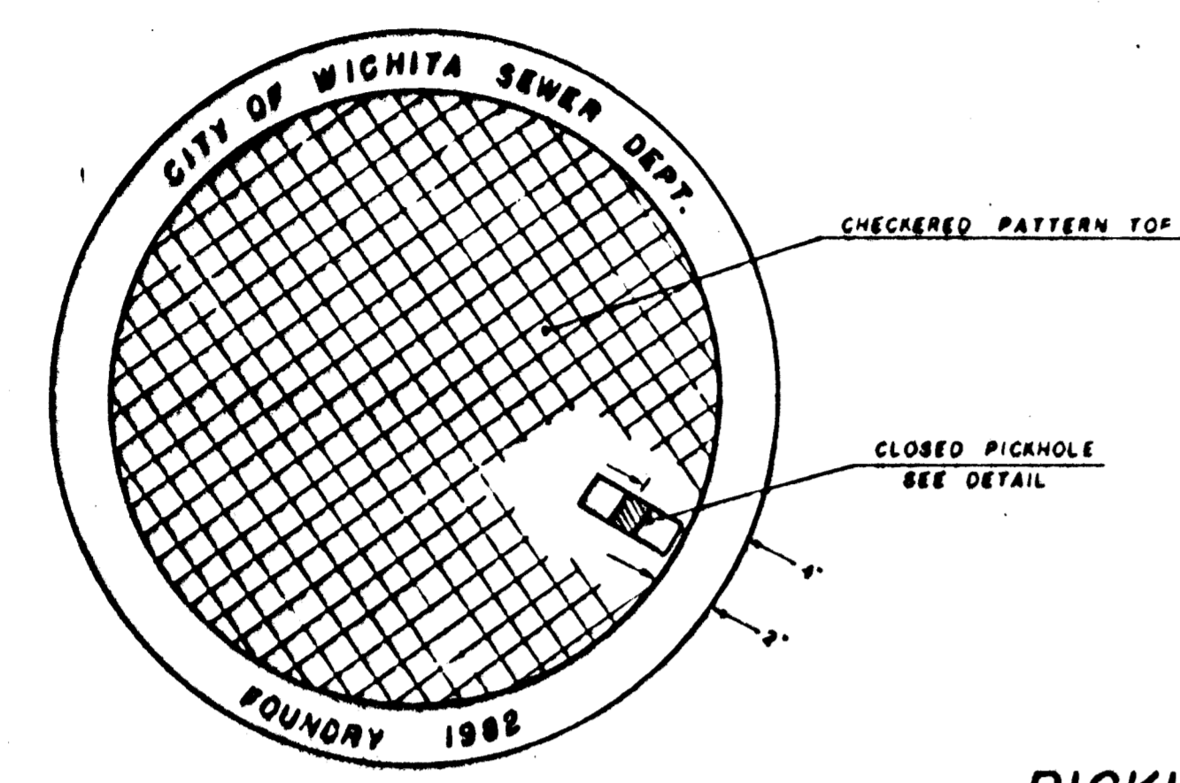
TOP VIEW
