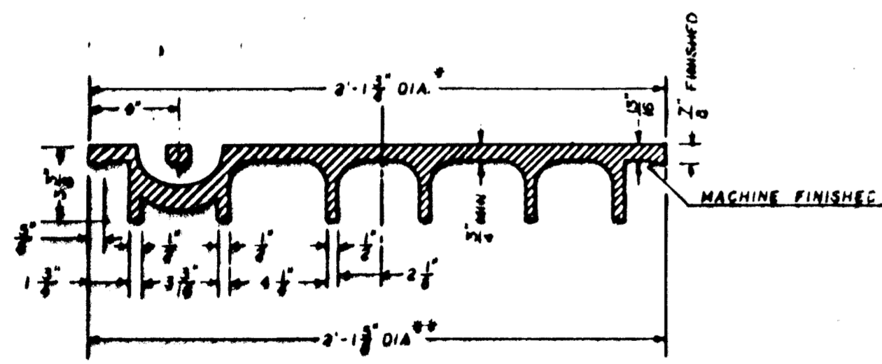
SECTION VIEW
