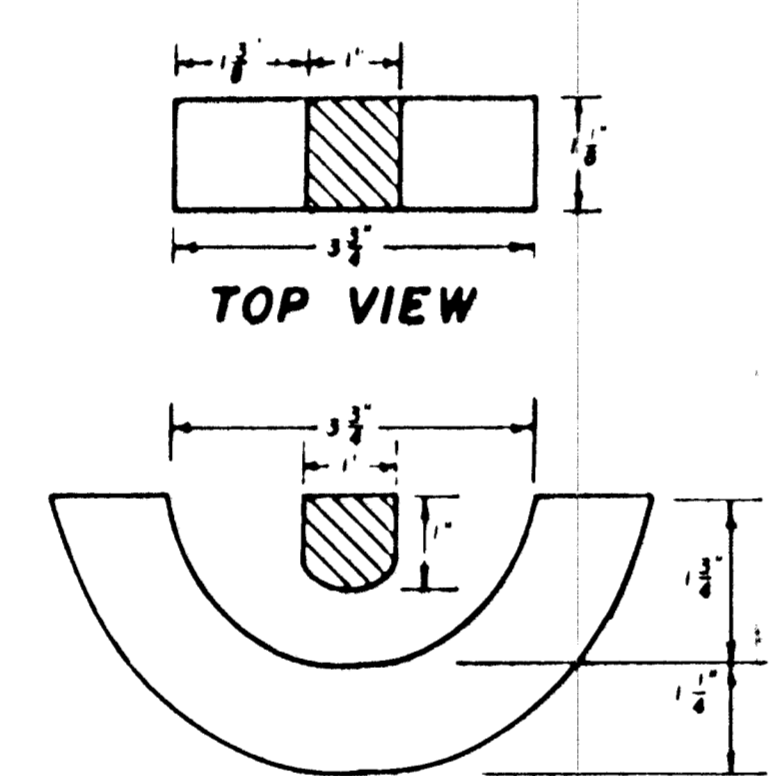
SECTION VIEW
